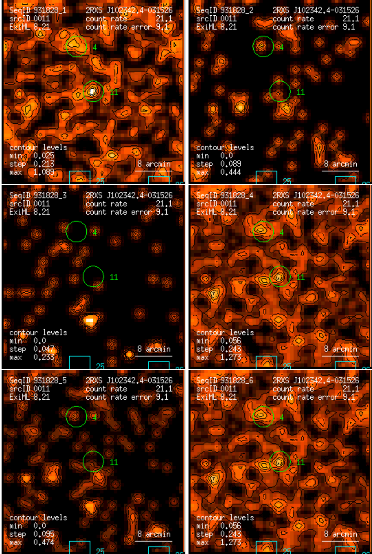
Figure 11: RASS 931828: detection 0011: band rate images, Gaussian filter: (1) PSPC channels 11 – 41, (2) 52 – 90, (3) 91 – 201, (4) 11 – 235, (5) 52 – 201, (6) 11 – 201. Broad band rates in counts/ks. Band rate contour levels in counts/ks/arcmin 2 .
