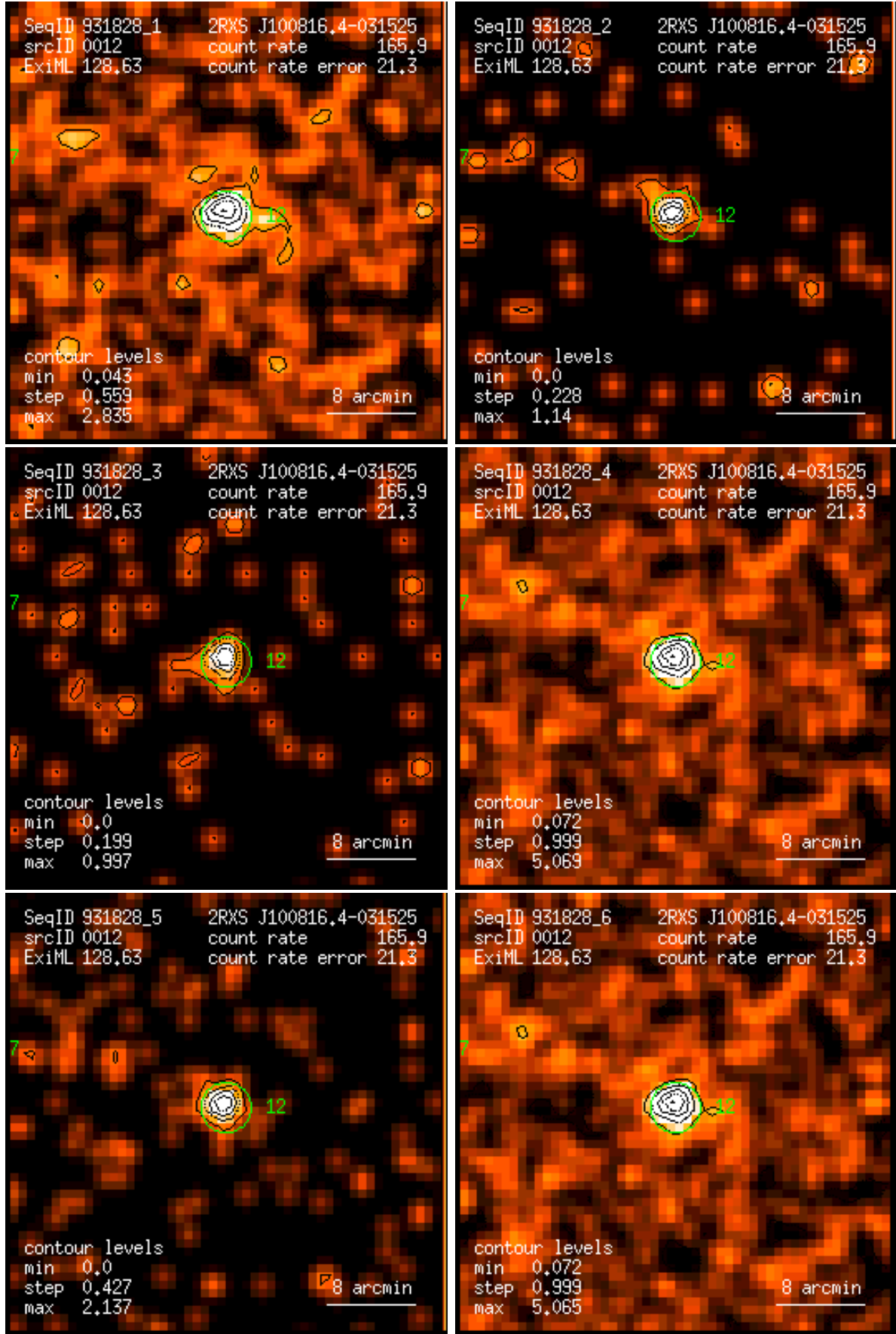
Figure 12: RASS 931828: detection 0012: band rate images, Gaussian filter: (1) PSPC channels 11 – 41, (2) 52 – 90, (3) 91 – 201, (4) 11 – 235, (5) 52 – 201, (6) 11 – 201. Broad band rates in counts/ks. Band rate contour levels in counts/ks/arcmin 2 .
