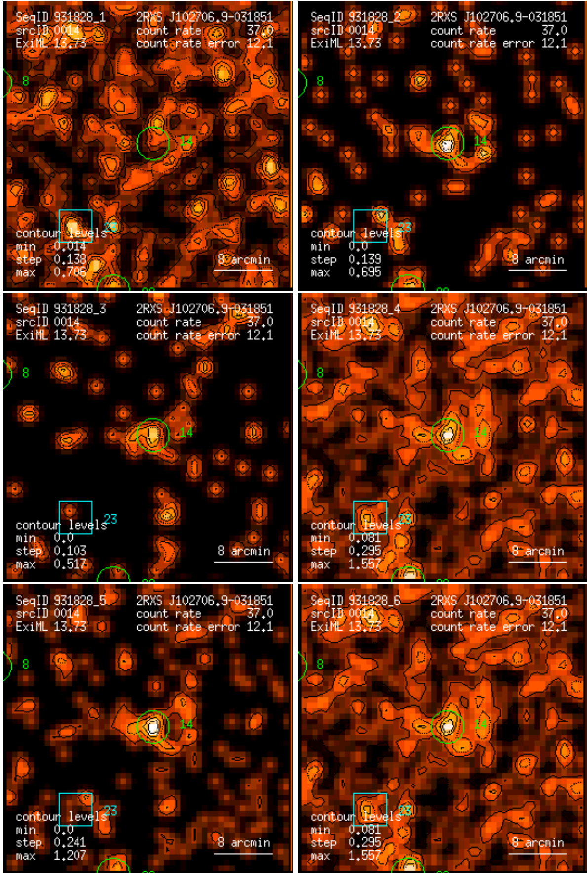
Figure 14: RASS 931828: detection 0014: band rate images, Gaussian filter: (1) PSPC channels 11 – 41, (2) 52 – 90, (3) 91 – 201, (4) 11 – 235, (5) 52 – 201, (6) 11 – 201. Broad band rates in counts/ks. Band rate contour levels in counts/ks/arcmin 2 .
