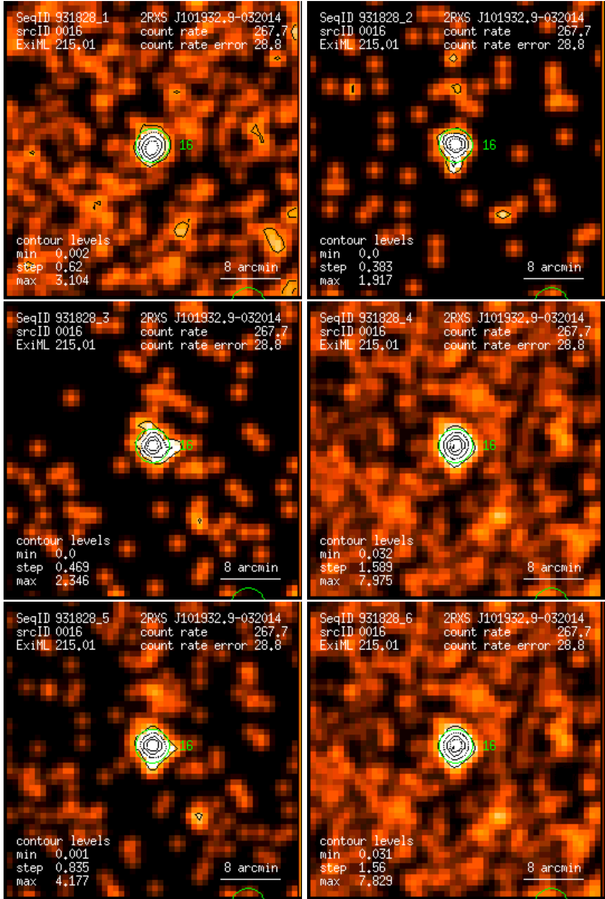
Figure 16: RASS 931828: detection 0016: band rate images, Gaussian filter: (1) PSPC channels 11 – 41, (2) 52 – 90, (3) 91 – 201, (4) 11 – 235, (5) 52 – 201, (6) 11 – 201. Broad band rates in counts/ks. Band rate contour levels in counts/ks/arcmin 2 .
