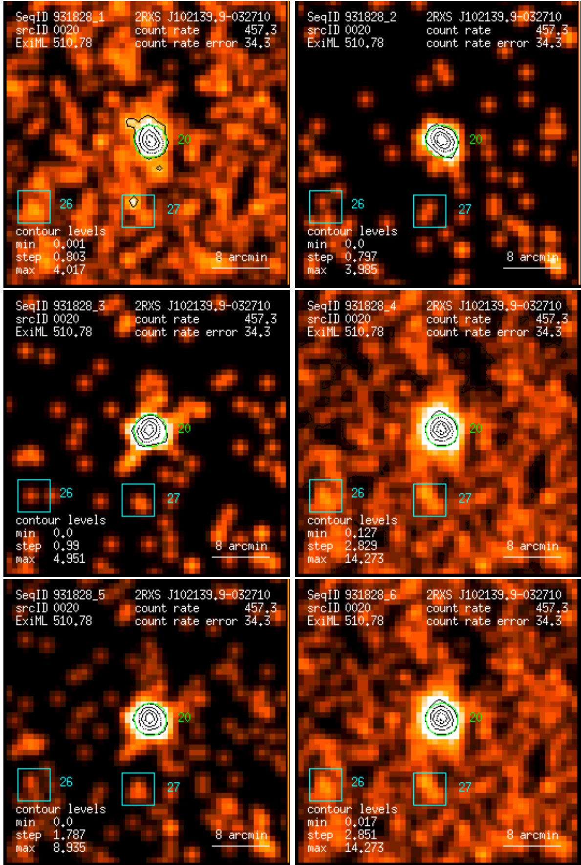
Figure 20: RASS 931828: detection 0020: band rate images, Gaussian filter: (1) PSPC channels 11 – 41, (2) 52 – 90, (3) 91 – 201, (4) 11 – 235, (5) 52 – 201, (6) 11 – 201. Broad band rates in counts/ks. Band rate contour levels in counts/ks/arcmin 2 .
