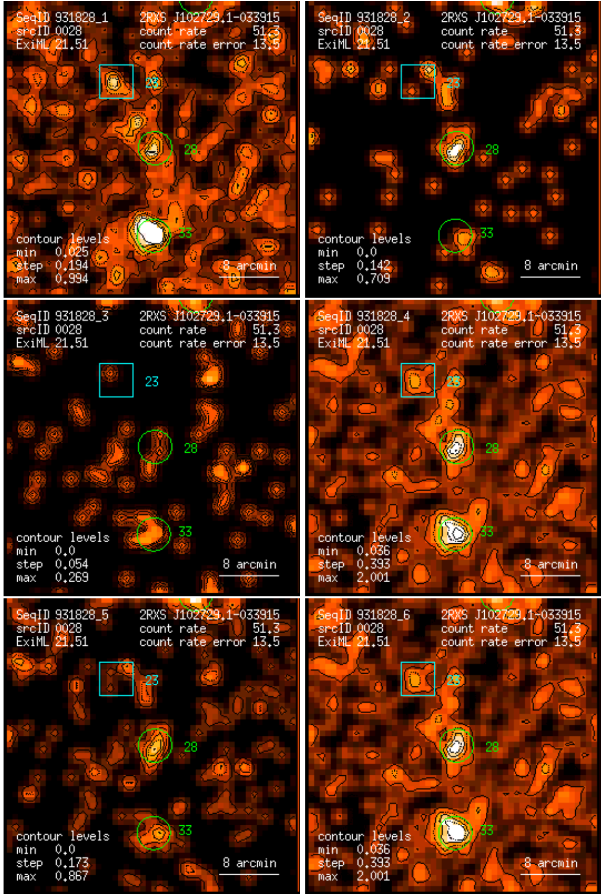
Figure 28: RASS 931828: detection 0028: band rate images, Gaussian filter: (1) PSPC channels 11 – 41, (2) 52 – 90, (3) 91 – 201, (4) 11 – 235, (5) 52 – 201, (6) 11 – 201. Broad band rates in counts/ks. Band rate contour levels in counts/ks/arcmin 2 .
