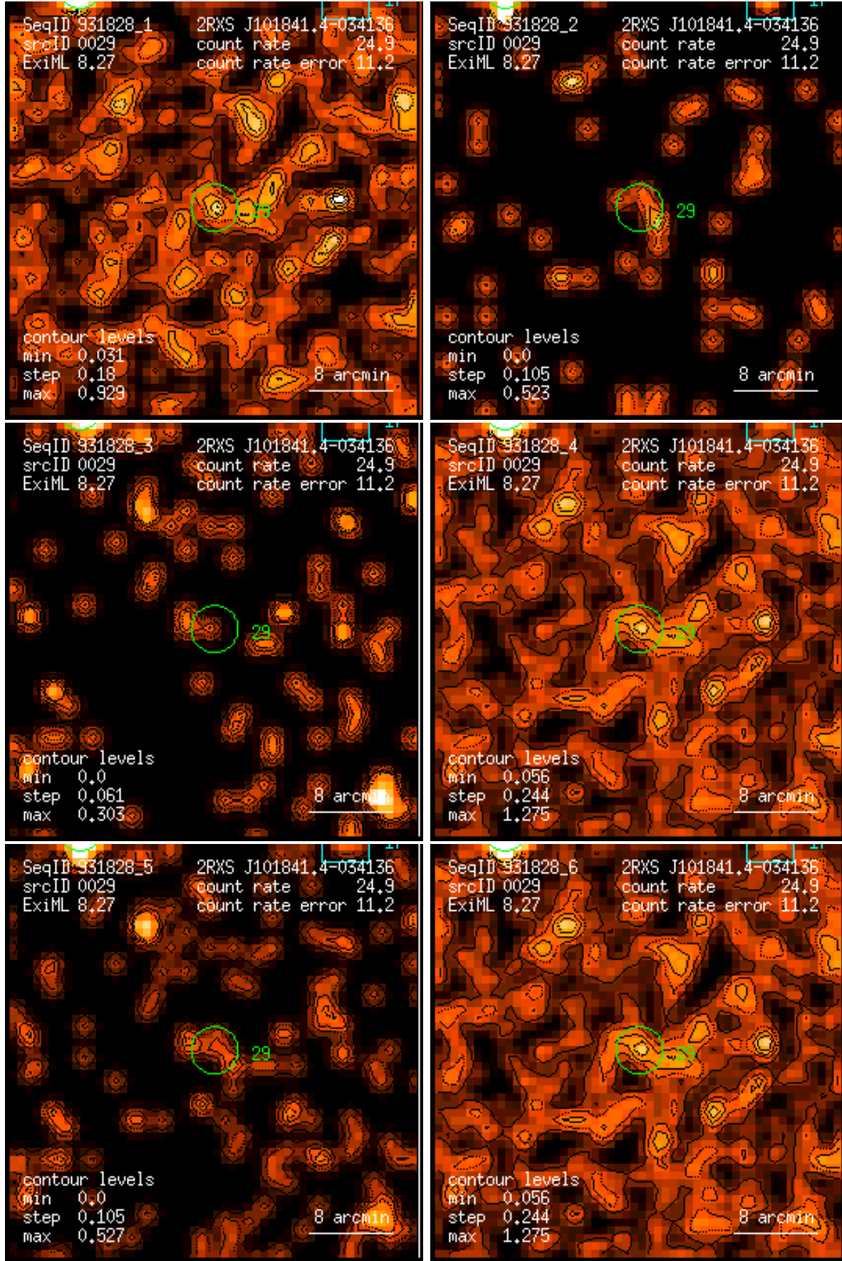
Figure 29: RASS 931828: detection 0029: band rate images, Gaussian filter: (1) PSPC channels 11 – 41, (2) 52 – 90, (3) 91 – 201, (4) 11 – 235, (5) 52 – 201, (6) 11 – 201. Broad band rates in counts/ks. Band rate contour levels in counts/ks/arcmin 2 .
