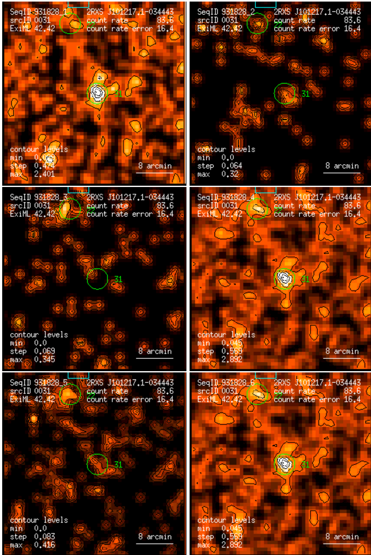
Figure 31: RASS 931828: detection 0031: band rate images, Gaussian filter: (1) PSPC channels 11 – 41, (2) 52 – 90, (3) 91 – 201, (4) 11 – 235, (5) 52 – 201, (6) 11 – 201. Broad band rates in counts/ks. Band rate contour levels in counts/ks/arcmin 2 .
