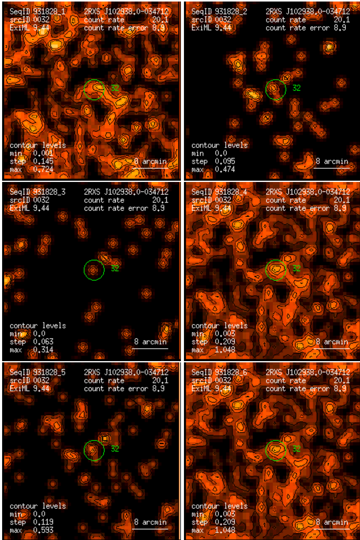
Figure 32: RASS 931828: detection 0032: band rate images, Gaussian filter: (1) PSPC channels 11 – 41, (2) 52 – 90, (3) 91 – 201, (4) 11 – 235, (5) 52 – 201, (6) 11 – 201. Broad band rates in counts/ks. Band rate contour levels in counts/ks/arcmin 2 .
