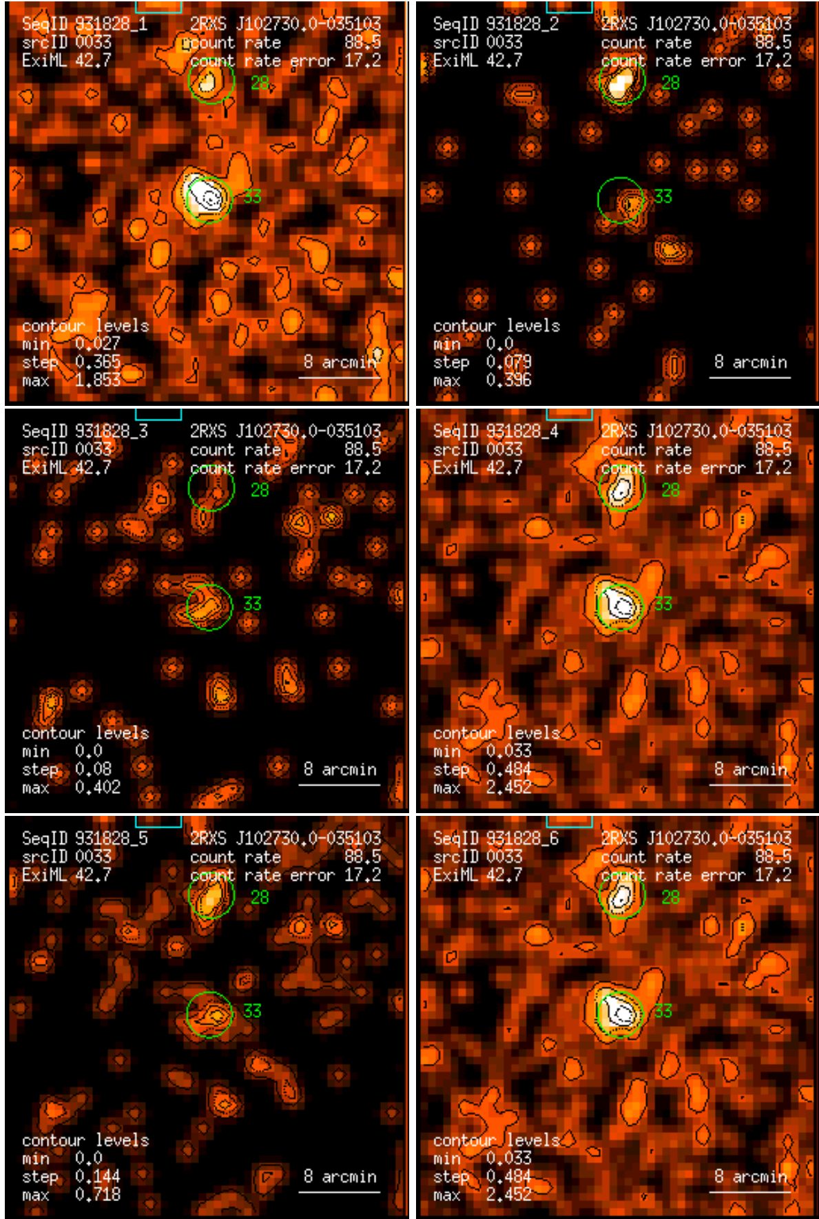
Figure 33: RASS 931828: detection 0033: band rate images, Gaussian filter: (1) PSPC channels 11 – 41, (2) 52 – 90, (3) 91 – 201, (4) 11 – 235, (5) 52 – 201, (6) 11 – 201. Broad band rates in counts/ks. Band rate contour levels in counts/ks/arcmin 2 .
