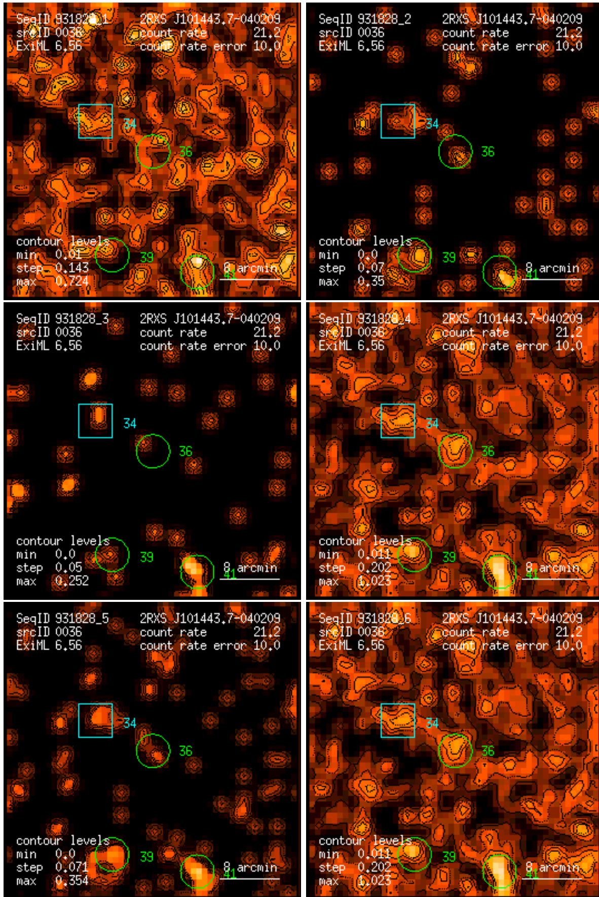
Figure 36: RASS 931828: detection 0036: band rate images, Gaussian filter: (1) PSPC channels 11 – 41, (2) 52 – 90, (3) 91 – 201, (4) 11 – 235, (5) 52 – 201, (6) 11 – 201. Broad band rates in counts/ks. Band rate contour levels in counts/ks/arcmin 2 .
