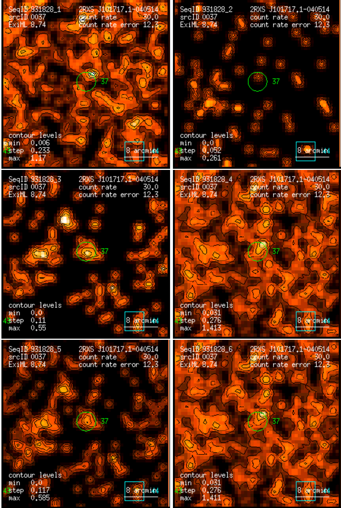
Figure 37: RASS 931828: detection 0037: band rate images, Gaussian filter: (1) PSPC channels 11 – 41, (2) 52 – 90, (3) 91 – 201, (4) 11 – 235, (5) 52 – 201, (6) 11 – 201. Broad band rates in counts/ks. Band rate contour levels in counts/ks/arcmin 2 .
