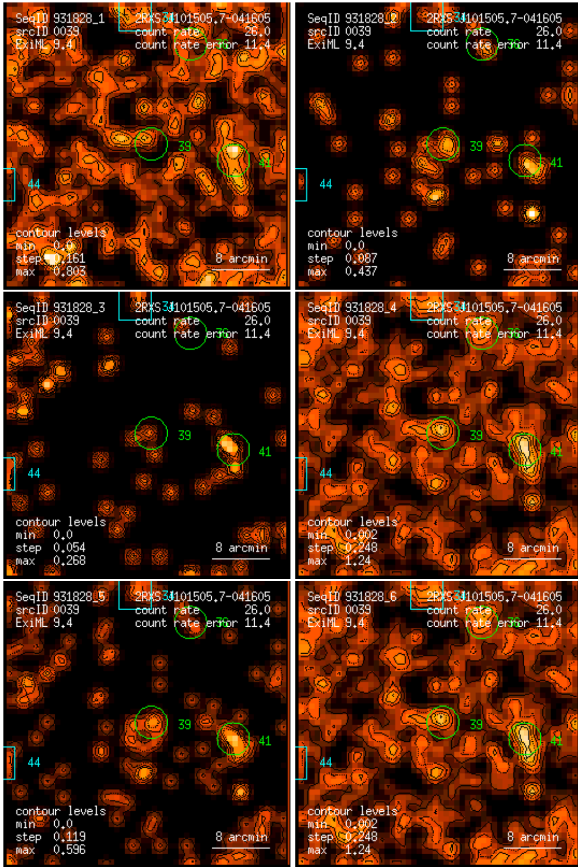
Figure 39: RASS 931828: detection 0039: band rate images, Gaussian filter: (1) PSPC channels 11 – 41, (2) 52 – 90, (3) 91 – 201, (4) 11 – 235, (5) 52 – 201, (6) 11 – 201. Broad band rates in counts/ks. Band rate contour levels in counts/ks/arcmin 2 .
