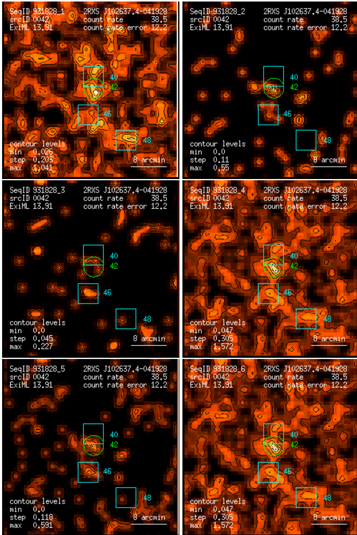
Figure 42: RASS 931828: detection 0042: band rate images, Gaussian filter: (1) PSPC channels 11 – 41, (2) 52 – 90, (3) 91 – 201, (4) 11 – 235, (5) 52 – 201, (6) 11 – 201. Broad band rates in counts/ks. Band rate contour levels in counts/ks/arcmin 2 .
