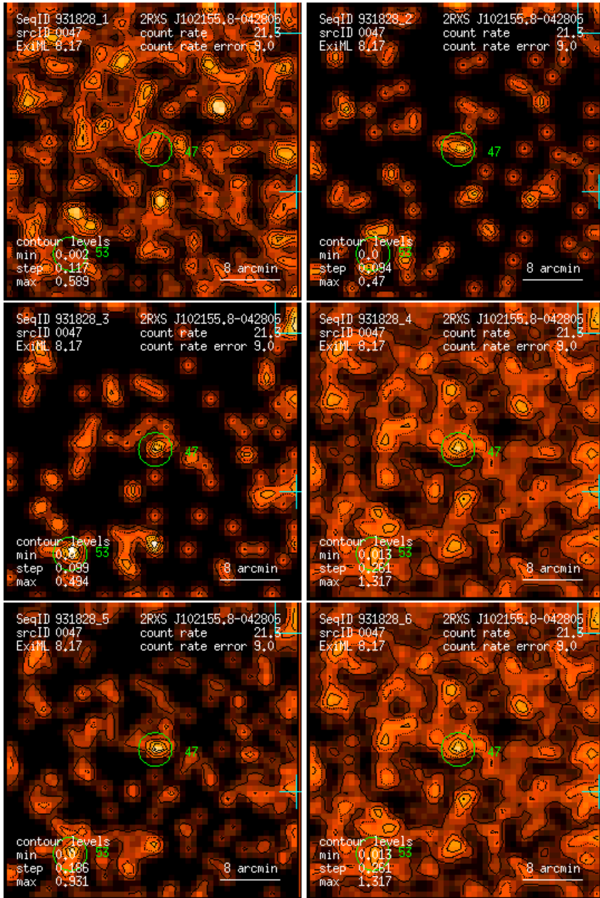
Figure 47: RASS 931828: detection 0047: band rate images, Gaussian filter: (1) PSPC channels 11 – 41, (2) 52 – 90, (3) 91 – 201, (4) 11 – 235, (5) 52 – 201, (6) 11 – 201. Broad band rates in counts/ks. Band rate contour levels in counts/ks/arcmin 2 .
