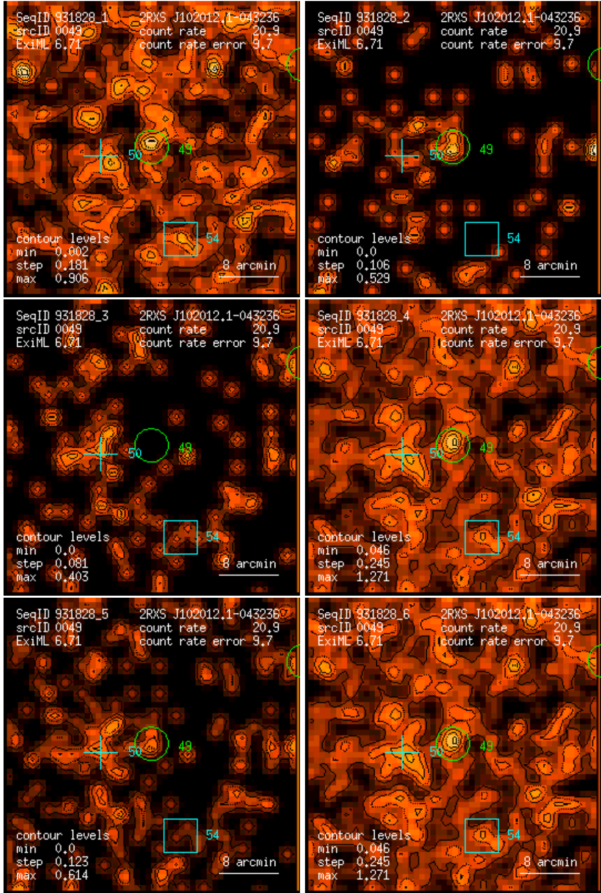
Figure 49: RASS 931828: detection 0049: band rate images, Gaussian filter: (1) PSPC channels 11 – 41, (2) 52 – 90, (3) 91 – 201, (4) 11 – 235, (5) 52 – 201, (6) 11 – 201. Broad band rates in counts/ks. Band rate contour levels in counts/ks/arcmin 2 .
