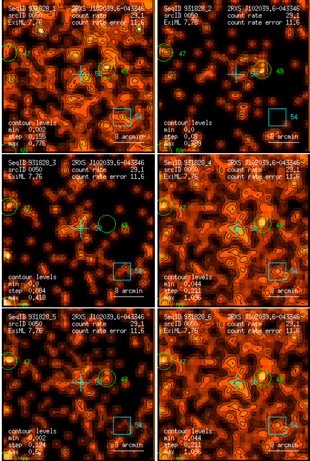
Figure 50: RASS 931828: detection 0050: band rate images, Gaussian filter: (1) PSPC channels 11 – 41, (2) 52 – 90, (3) 91 – 201, (4) 11 – 235, (5) 52 – 201, (6) 11 – 201. Broad band rates in counts/ks. Band rate contour levels in counts/ks/arcmin 2 .
