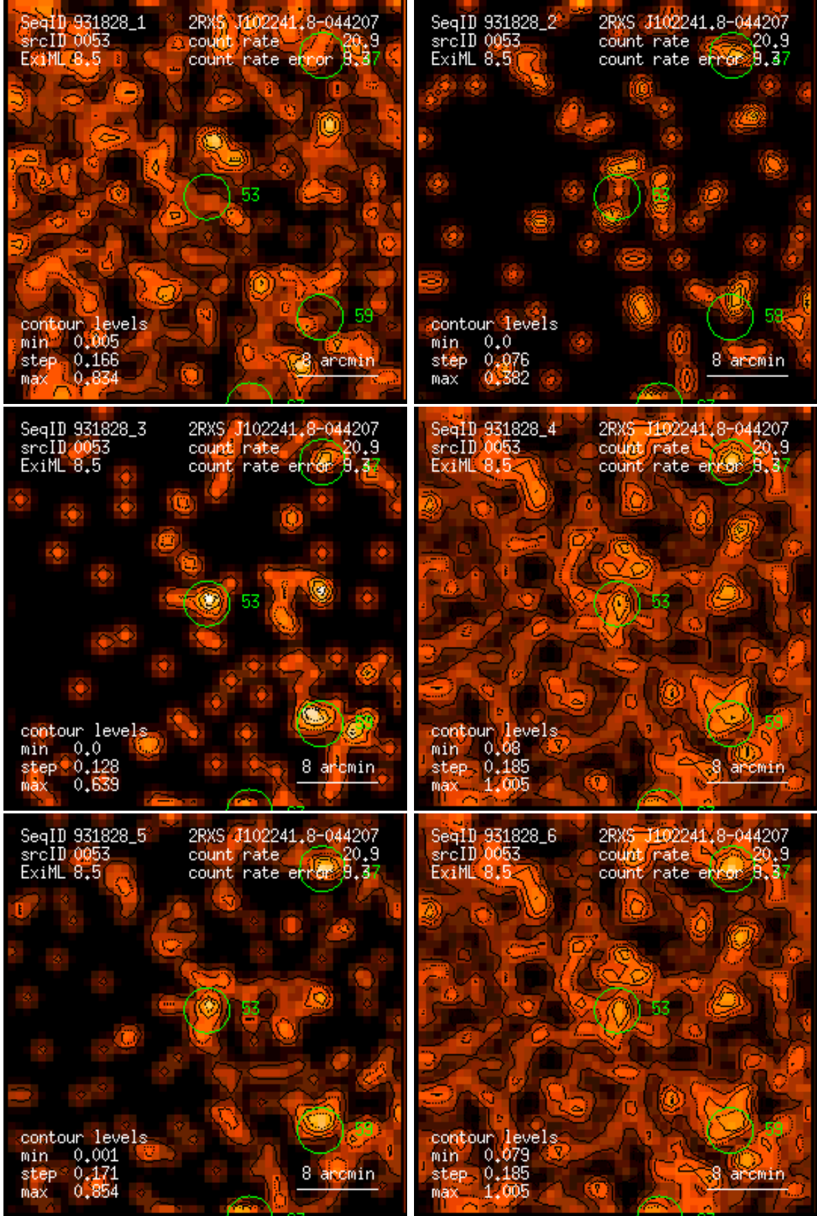
Figure 53: RASS 931828: detection 0053: band rate images, Gaussian filter: (1) PSPC channels 11 – 41, (2) 52 – 90, (3) 91 – 201, (4) 11 – 235, (5) 52 – 201, (6) 11 – 201. Broad band rates in counts/ks. Band rate contour levels in counts/ks/arcmin 2 .
