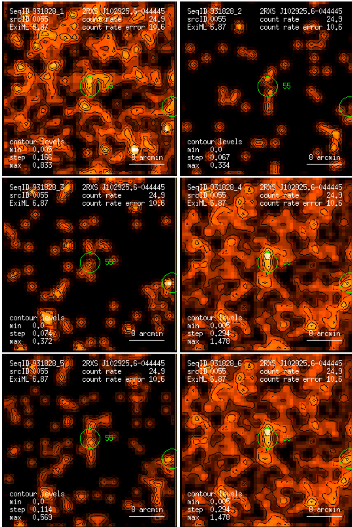
Figure 55: RASS 931828: detection 0055: band rate images, Gaussian filter: (1) PSPC channels 11 – 41, (2) 52 – 90, (3) 91 – 201, (4) 11 – 235, (5) 52 – 201, (6) 11 – 201. Broad band rates in counts/ks. Band rate contour levels in counts/ks/arcmin 2 .
