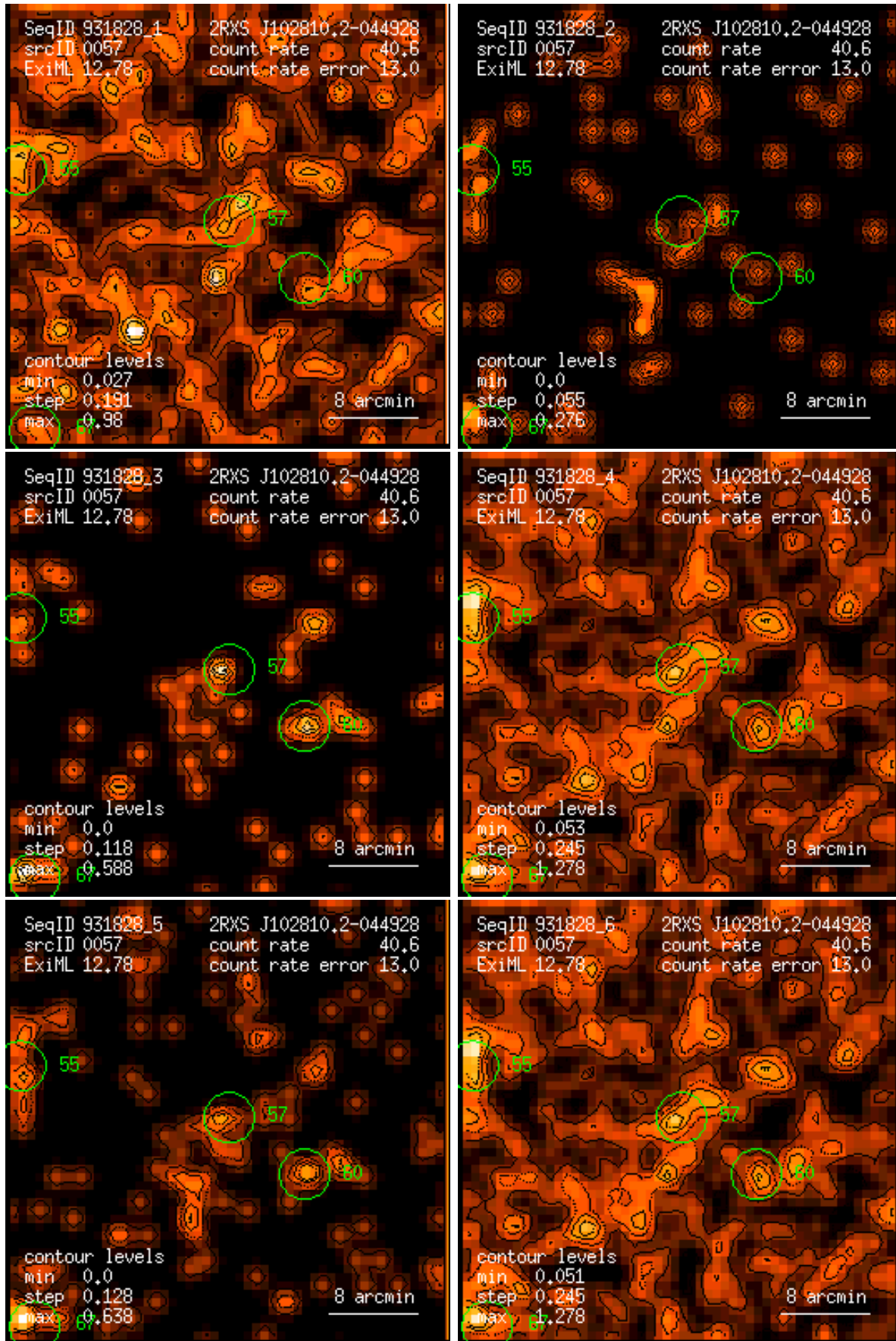
Figure 57: RASS 931828: detection 0057: band rate images, Gaussian filter: (1) PSPC channels 11 – 41, (2) 52 – 90, (3) 91 – 201, (4) 11 – 235, (5) 52 – 201, (6) 11 – 201. Broad band rates in counts/ks. Band rate contour levels in counts/ks/arcmin 2 .
