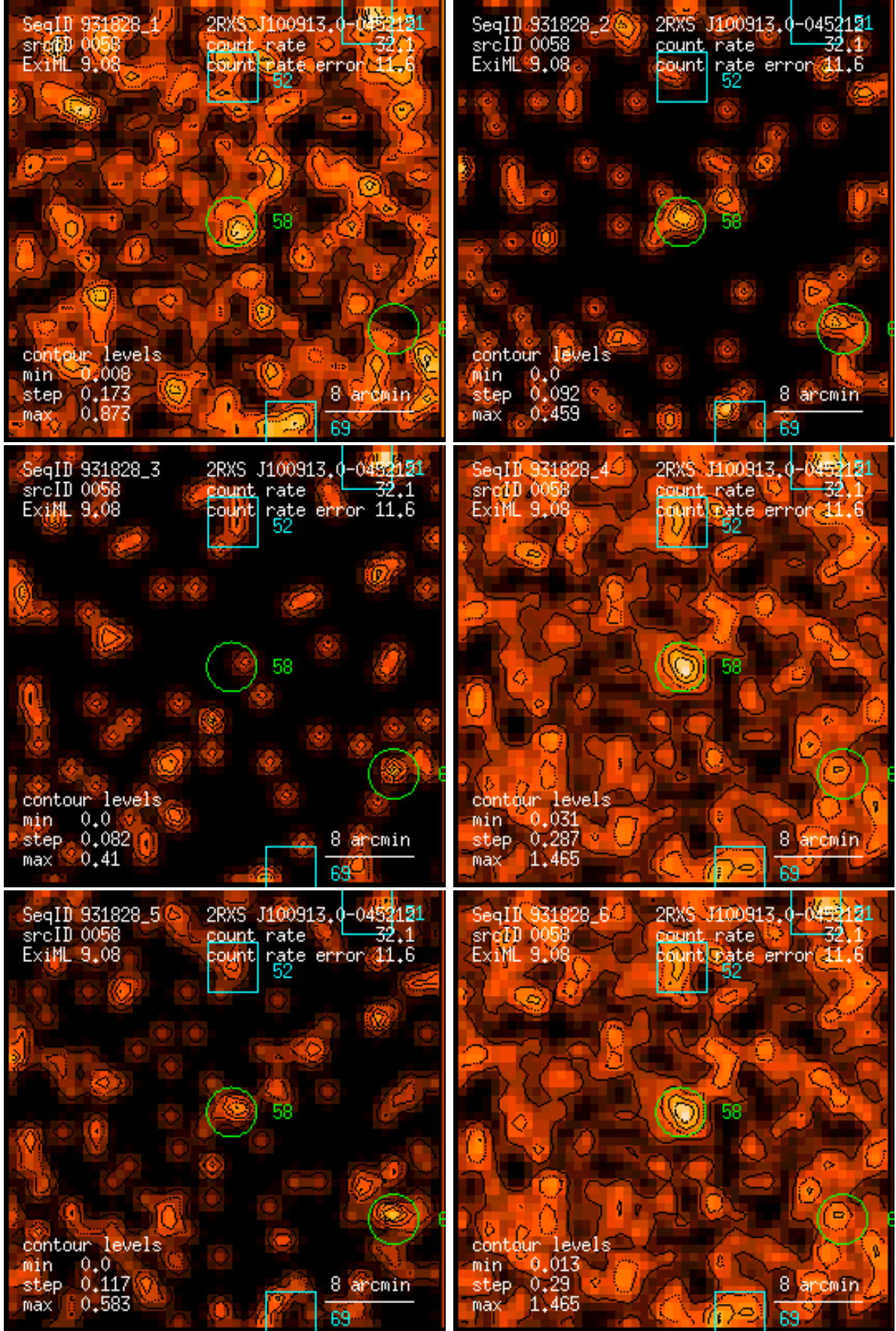
Figure 58: RASS 931828: detection 0058: band rate images, Gaussian filter: (1) PSPC channels 11 – 41, (2) 52 – 90, (3) 91 – 201, (4) 11 – 235, (5) 52 – 201, (6) 11 – 201. Broad band rates in counts/ks. Band rate contour levels in counts/ks/arcmin 2 .
