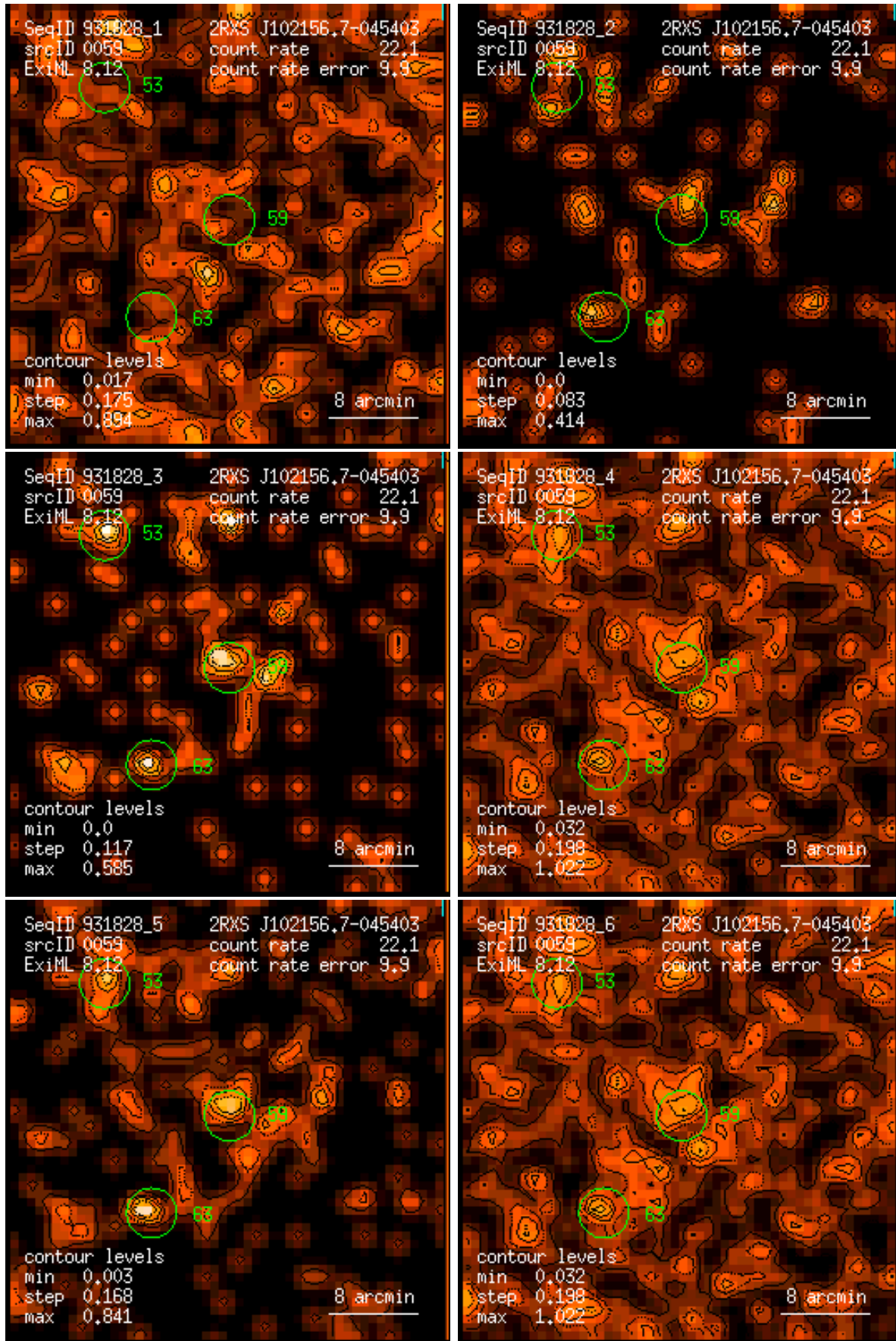
Figure 59: RASS 931828: detection 0059: band rate images, Gaussian filter: (1) PSPC channels 11 – 41, (2) 52 – 90, (3) 91 – 201, (4) 11 – 235, (5) 52 – 201, (6) 11 – 201. Broad band rates in counts/ks. Band rate contour levels in counts/ks/arcmin 2 .
