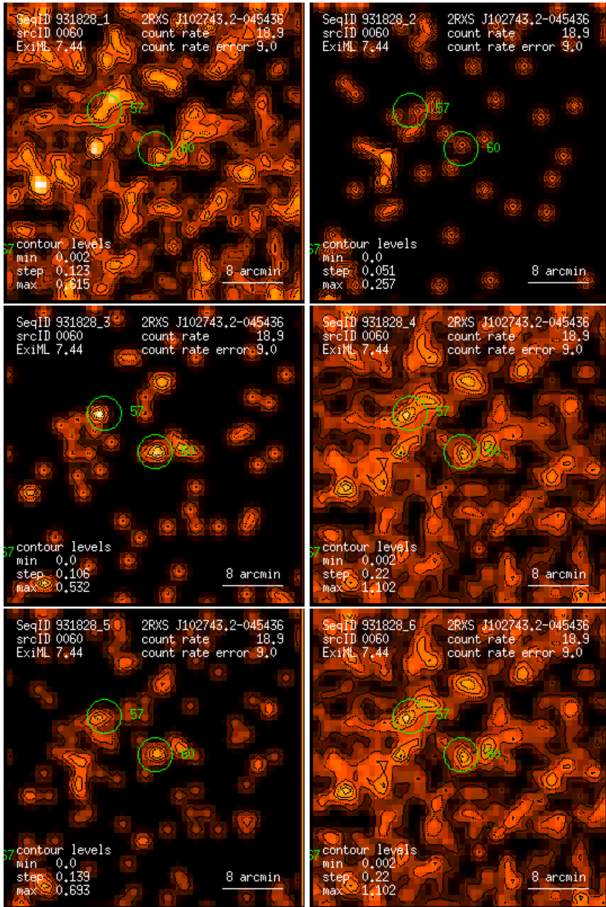
Figure 60: RASS 931828: detection 0060: band rate images, Gaussian filter: (1) PSPC channels 11 – 41, (2) 52 – 90, (3) 91 – 201, (4) 11 – 235, (5) 52 – 201, (6) 11 – 201. Broad band rates in counts/ks. Band rate contour levels in counts/ks/arcmin 2 .
