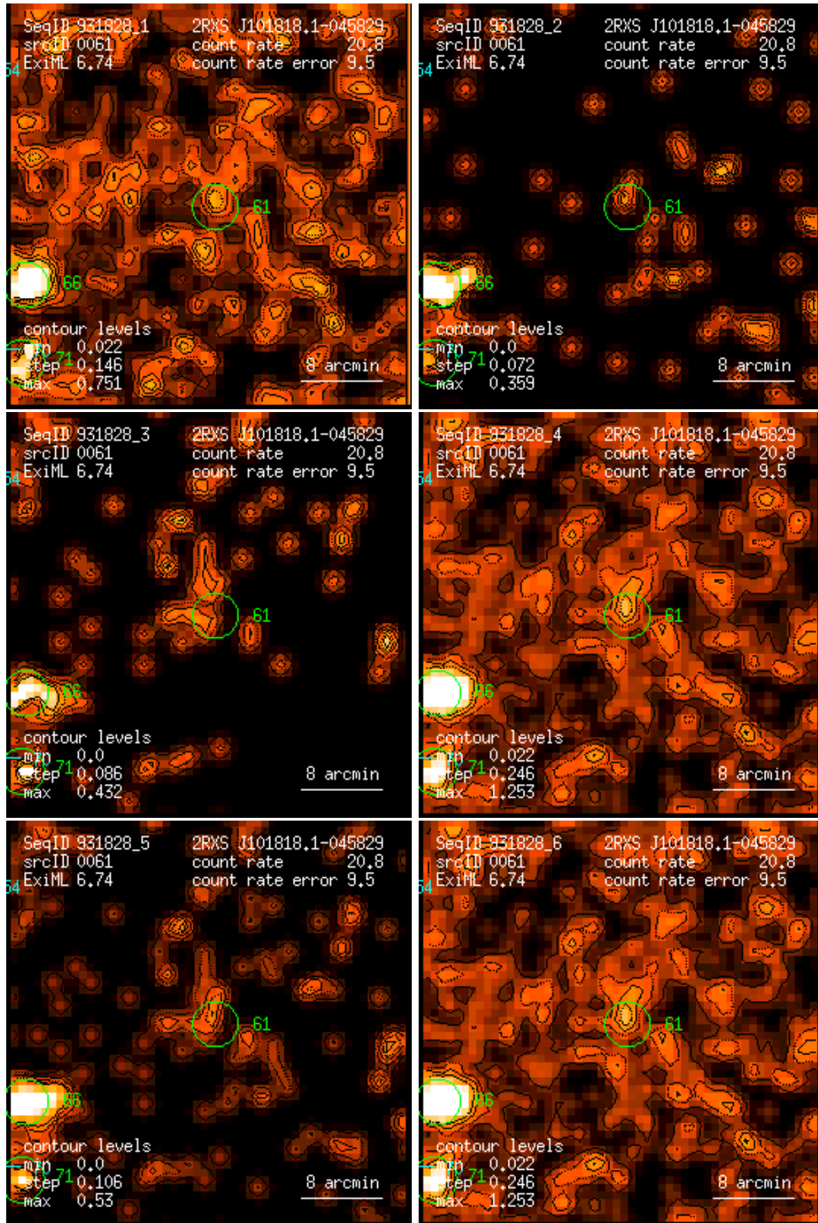
Figure 61: RASS 931828: detection 0061: band rate images, Gaussian filter: (1) PSPC channels 11 – 41, (2) 52 – 90, (3) 91 – 201, (4) 11 – 235, (5) 52 – 201, (6) 11 – 201. Broad band rates in counts/ks. Band rate contour levels in counts/ks/arcmin 2 .
