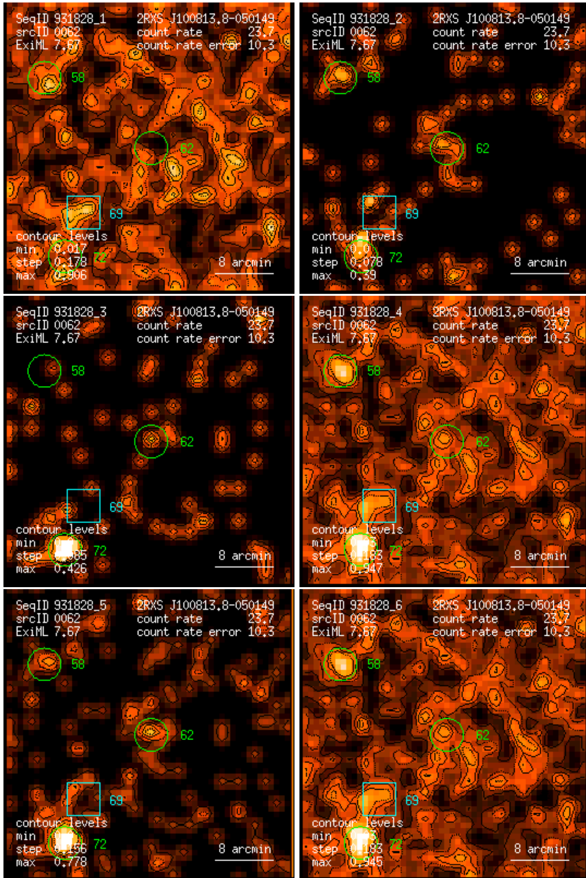
Figure 62: RASS 931828: detection 0062: band rate images, Gaussian filter: (1) PSPC channels 11 – 41, (2) 52 – 90, (3) 91 – 201, (4) 11 – 235, (5) 52 – 201, (6) 11 – 201. Broad band rates in counts/ks. Band rate contour levels in counts/ks/arcmin 2 .
