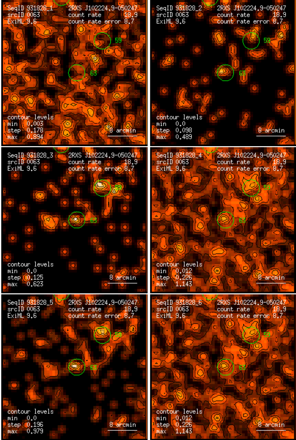
Figure 63: RASS 931828: detection 0063: band rate images, Gaussian filter: (1) PSPC channels 11 – 41, (2) 52 – 90, (3) 91 – 201, (4) 11 – 235, (5) 52 – 201, (6) 11 – 201. Broad band rates in counts/ks. Band rate contour levels in counts/ks/arcmin 2 .
