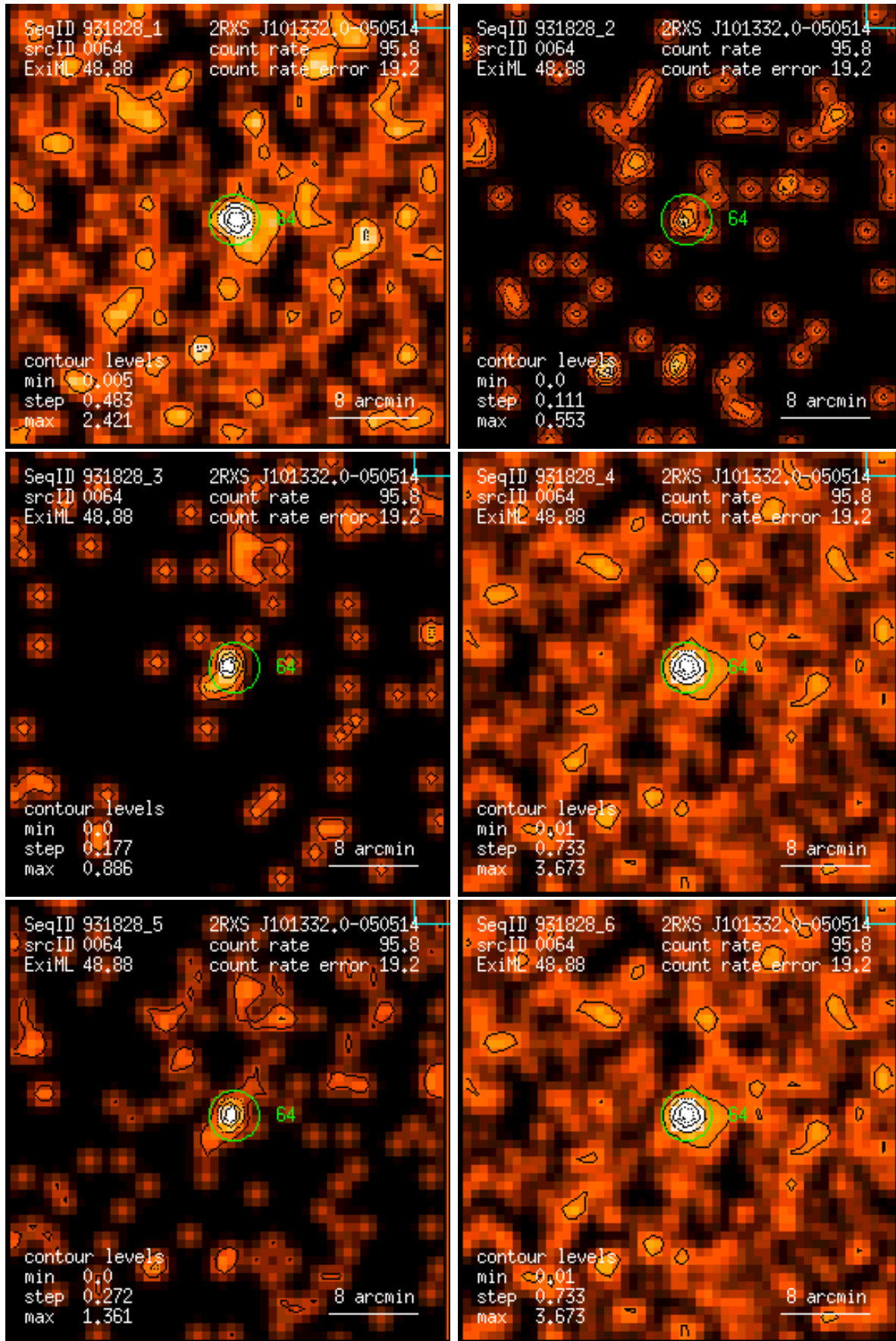
Figure 64: RASS 931828: detection 0064: band rate images, Gaussian filter: (1) PSPC channels 11 – 41, (2) 52 – 90, (3) 91 – 201, (4) 11 – 235, (5) 52 – 201, (6) 11 – 201. Broad band rates in counts/ks. Band rate contour levels in counts/ks/arcmin 2 .
