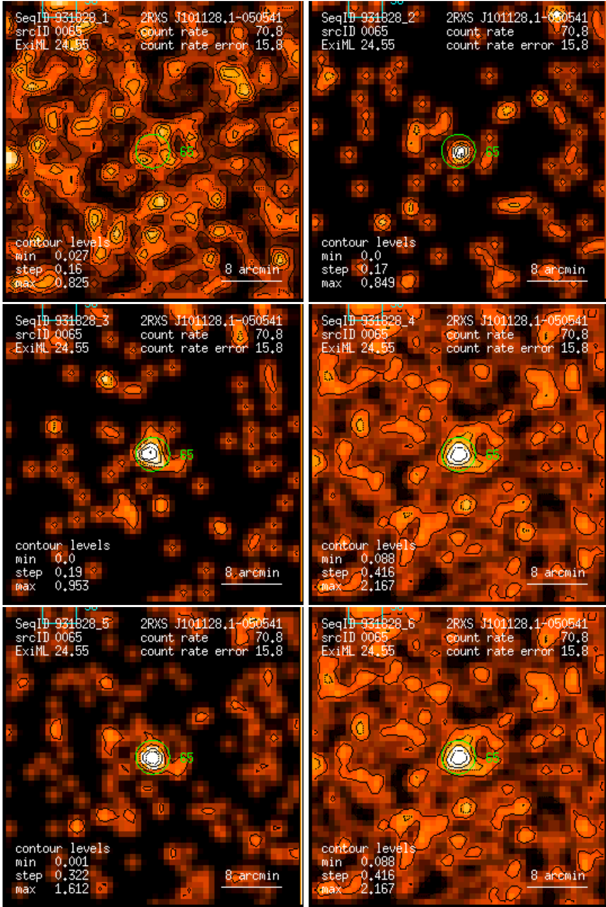
Figure 65: RASS 931828: detection 0065: band rate images, Gaussian filter: (1) PSPC channels 11 – 41, (2) 52 – 90, (3) 91 – 201, (4) 11 – 235, (5) 52 – 201, (6) 11 – 201. Broad band rates in counts/ks. Band rate contour levels in counts/ks/arcmin 2 .
