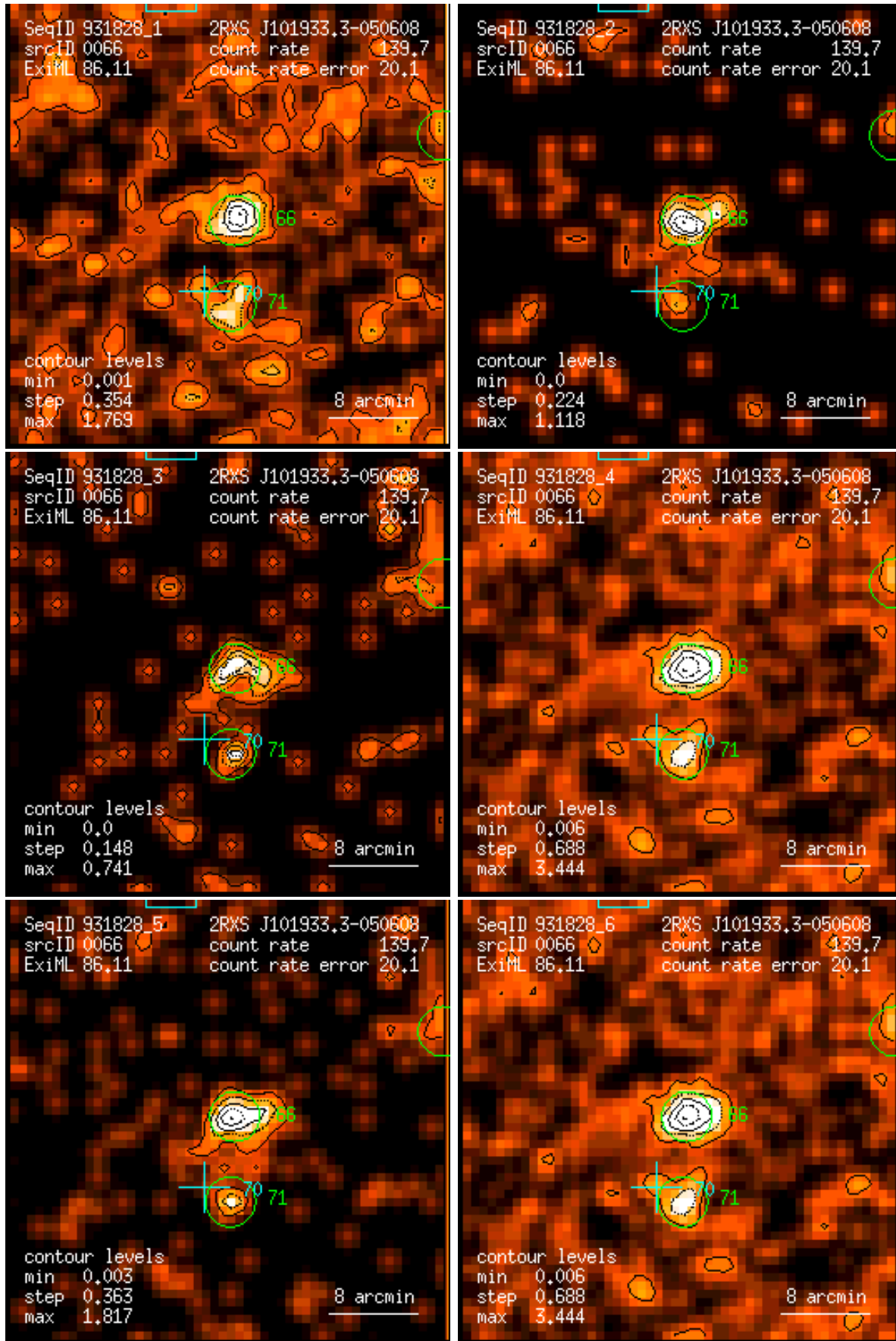
Figure 66: RASS 931828: detection 0066: band rate images, Gaussian filter: (1) PSPC channels 11 – 41, (2) 52 – 90, (3) 91 – 201, (4) 11 – 235, (5) 52 – 201, (6) 11 – 201. Broad band rates in counts/ks. Band rate contour levels in counts/ks/arcmin 2 .
