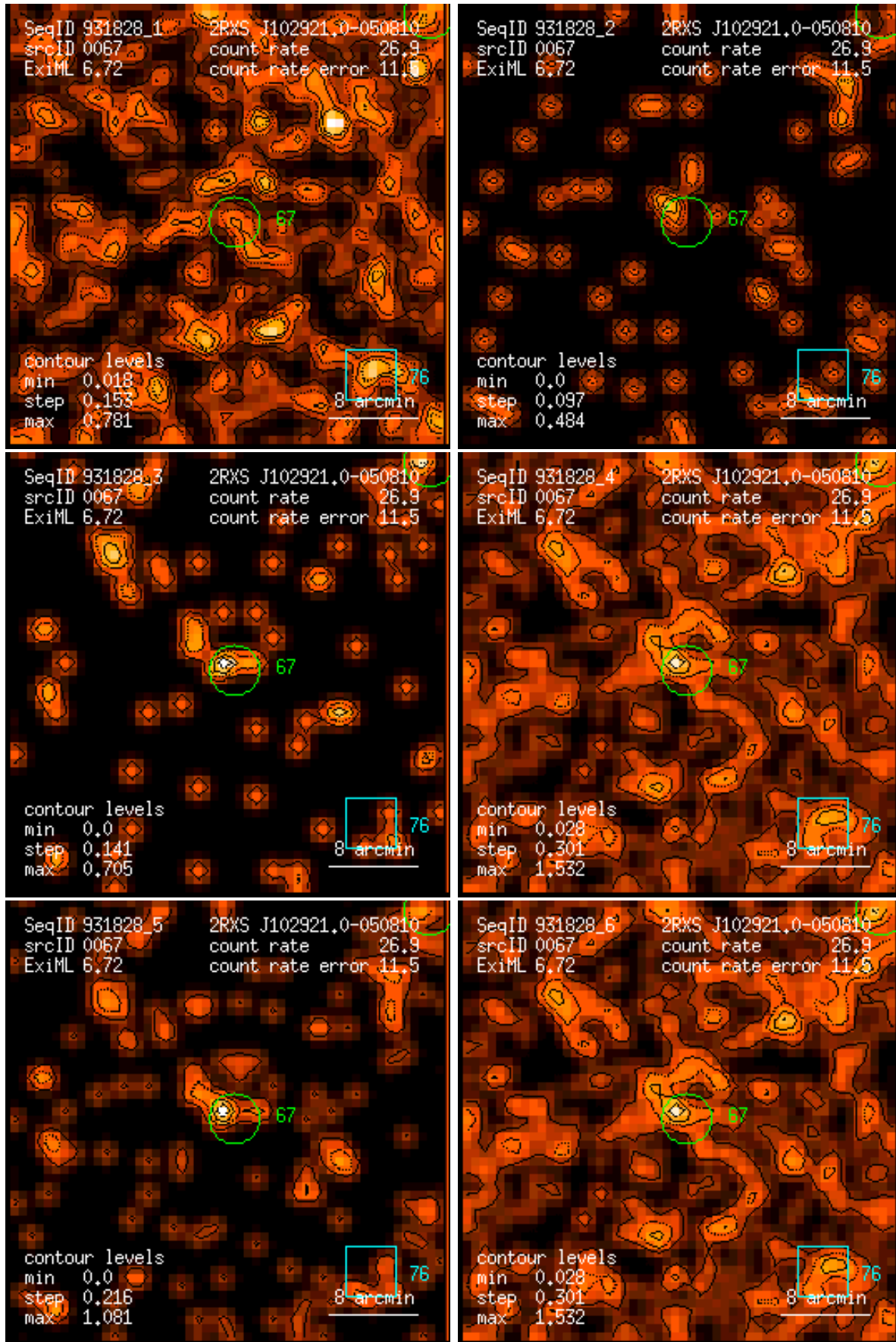
Figure 67: RASS 931828: detection 0067: band rate images, Gaussian filter: (1) PSPC channels 11 – 41, (2) 52 – 90, (3) 91 – 201, (4) 11 – 235, (5) 52 – 201, (6) 11 – 201. Broad band rates in counts/ks. Band rate contour levels in counts/ks/arcmin 2 .
