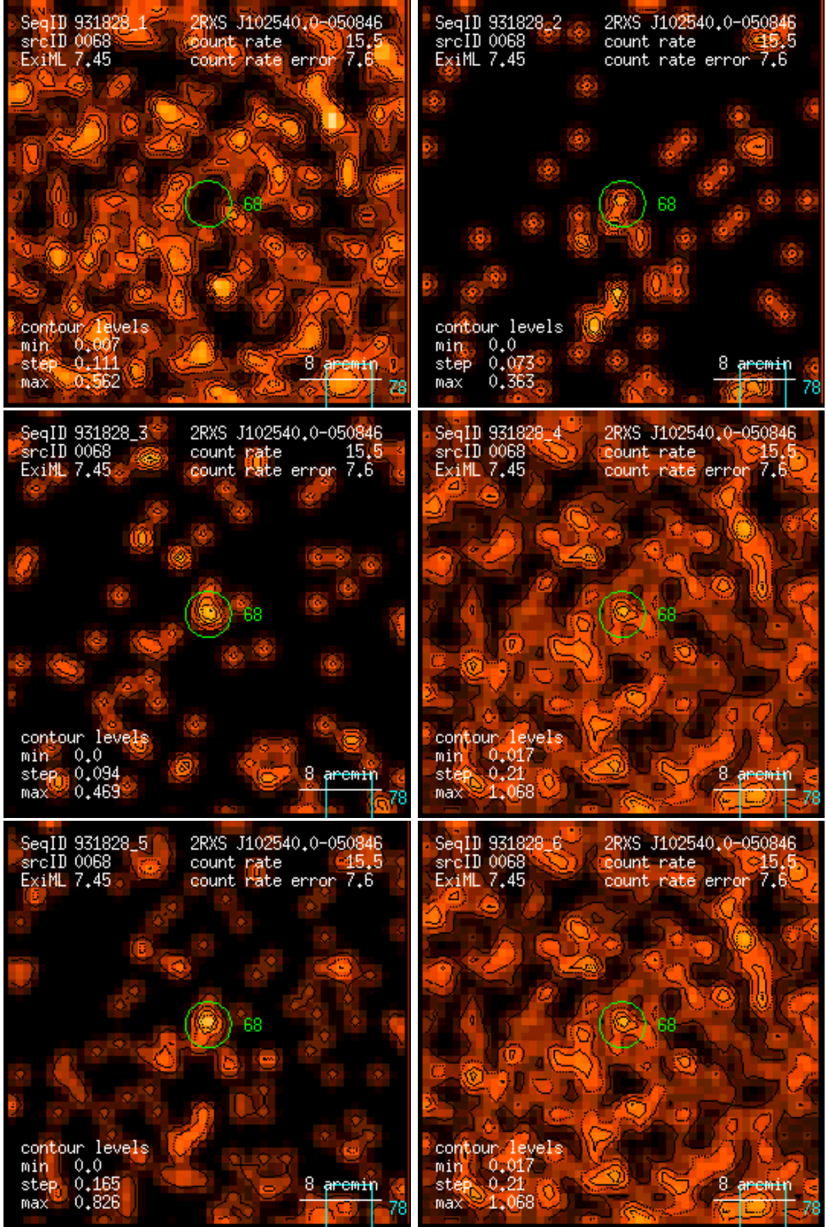
Figure 68: RASS 931828: detection 0068: band rate images, Gaussian filter: (1) PSPC channels 11 – 41, (2) 52 – 90, (3) 91 – 201, (4) 11 – 235, (5) 52 – 201, (6) 11 – 201. Broad band rates in counts/ks. Band rate contour levels in counts/ks/arcmin 2 .
