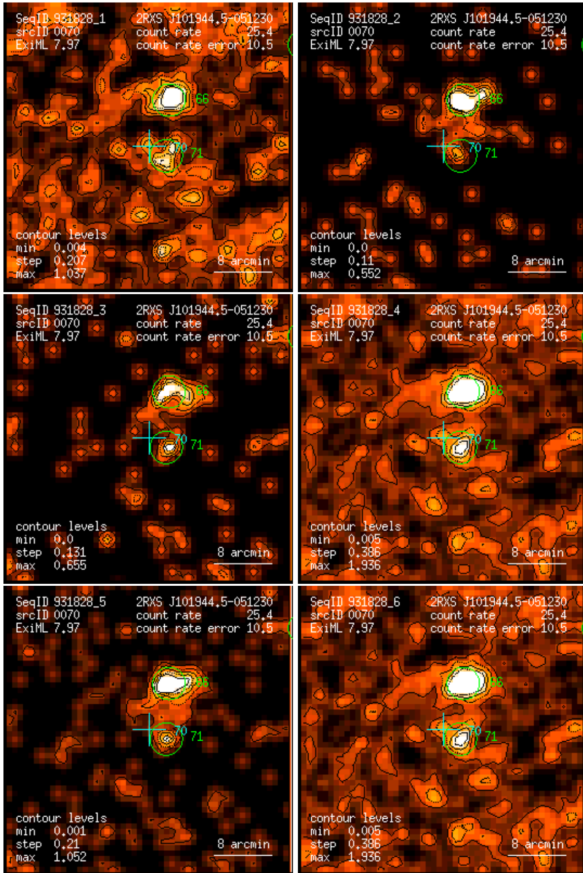
Figure 70: RASS 931828: detection 0070: band rate images, Gaussian filter: (1) PSPC channels 11 – 41, (2) 52 – 90, (3) 91 – 201, (4) 11 – 235, (5) 52 – 201, (6) 11 – 201. Broad band rates in counts/ks. Band rate contour levels in counts/ks/arcmin 2 .
