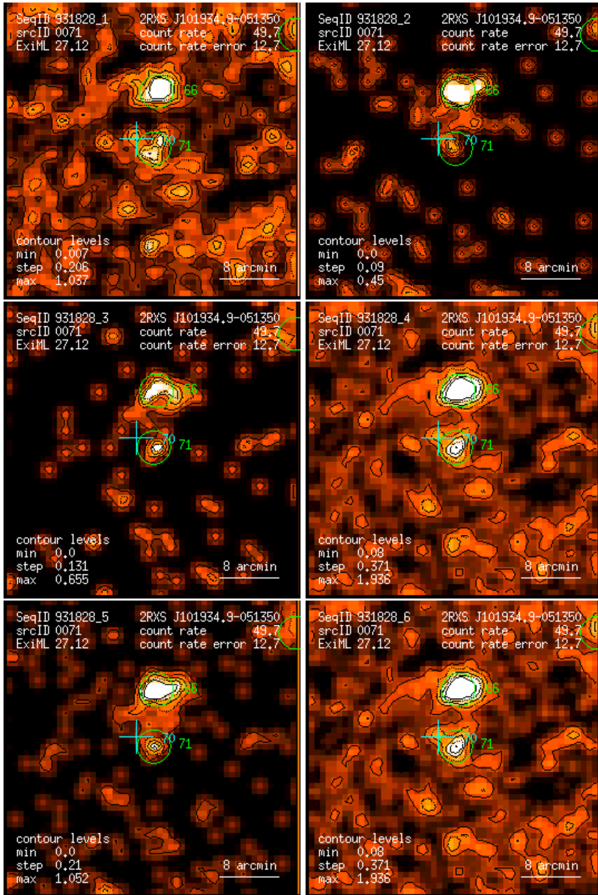
Figure 71: RASS 931828: detection 0071: band rate images, Gaussian filter: (1) PSPC channels 11 – 41, (2) 52 – 90, (3) 91 – 201, (4) 11 – 235, (5) 52 – 201, (6) 11 – 201. Broad band rates in counts/ks. Band rate contour levels in counts/ks/arcmin 2 .
