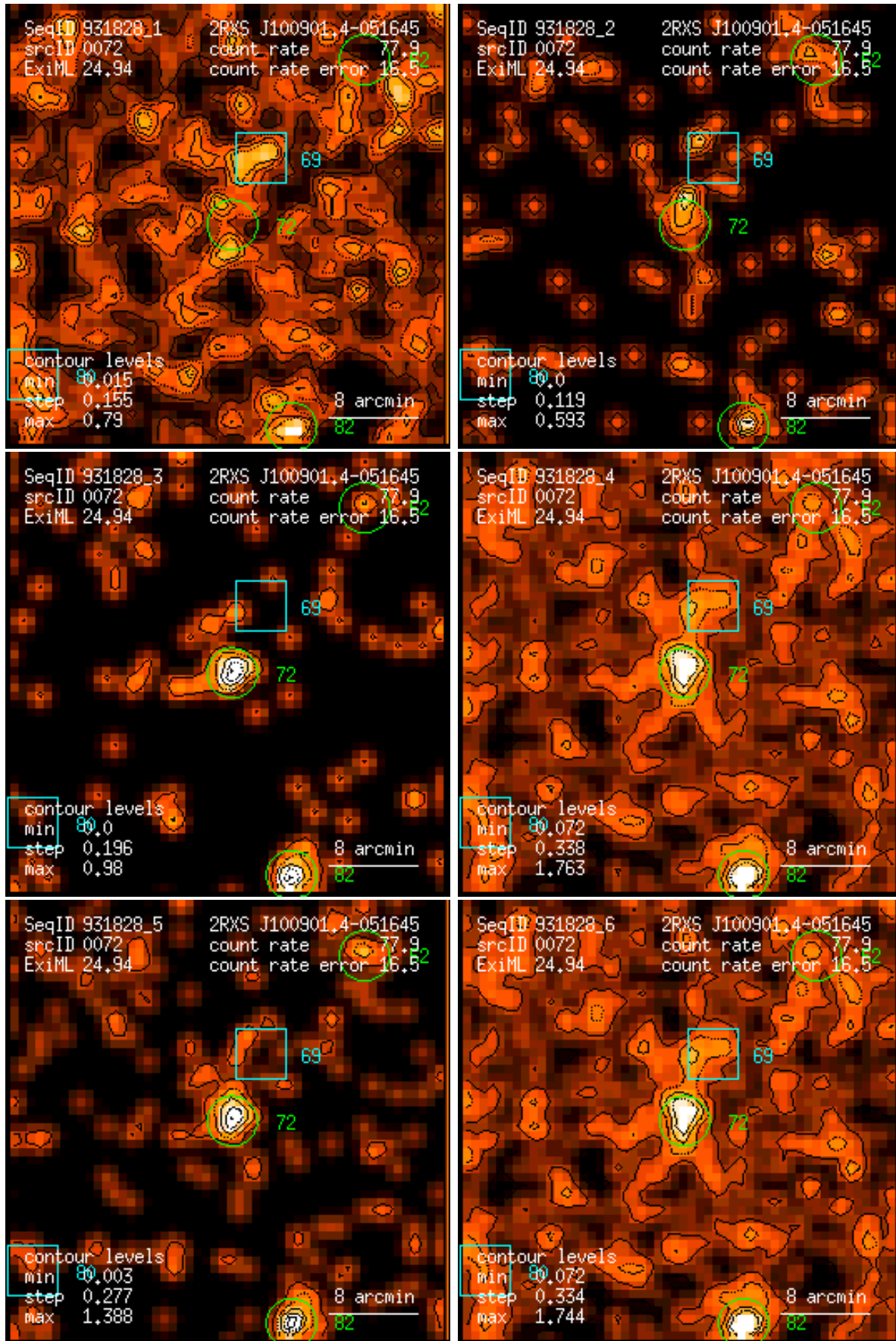
Figure 72: RASS 931828: detection 0072: band rate images, Gaussian filter: (1) PSPC channels 11 – 41, (2) 52 – 90, (3) 91 – 201, (4) 11 – 235, (5) 52 – 201, (6) 11 – 201. Broad band rates in counts/ks. Band rate contour levels in counts/ks/arcmin 2 .
