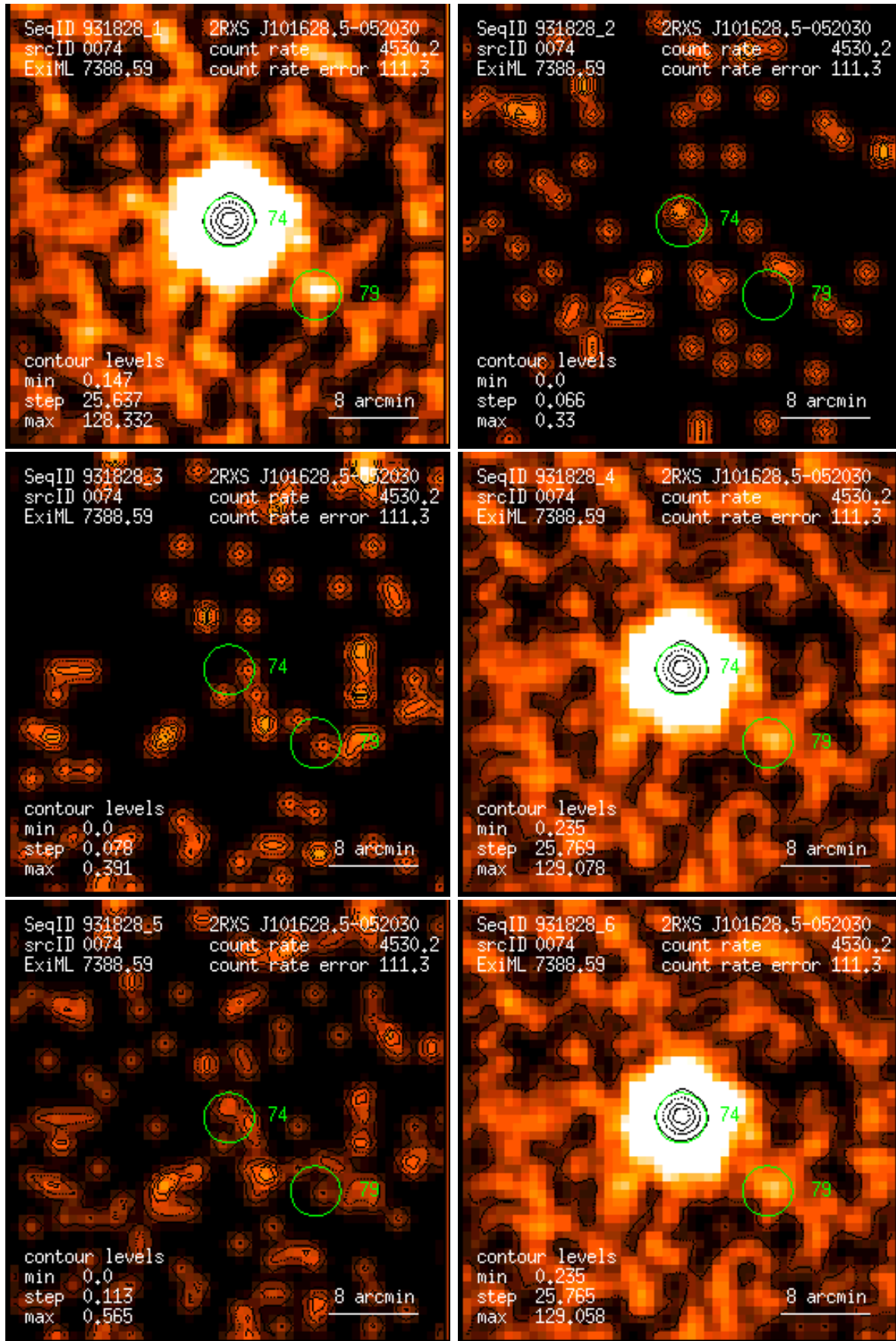
Figure 74: RASS 931828: detection 0074: band rate images, Gaussian filter: (1) PSPC channels 11 – 41, (2) 52 – 90, (3) 91 – 201, (4) 11 – 235, (5) 52 – 201, (6) 11 – 201. Broad band rates in counts/ks. Band rate contour levels in counts/ks/arcmin 2 .
