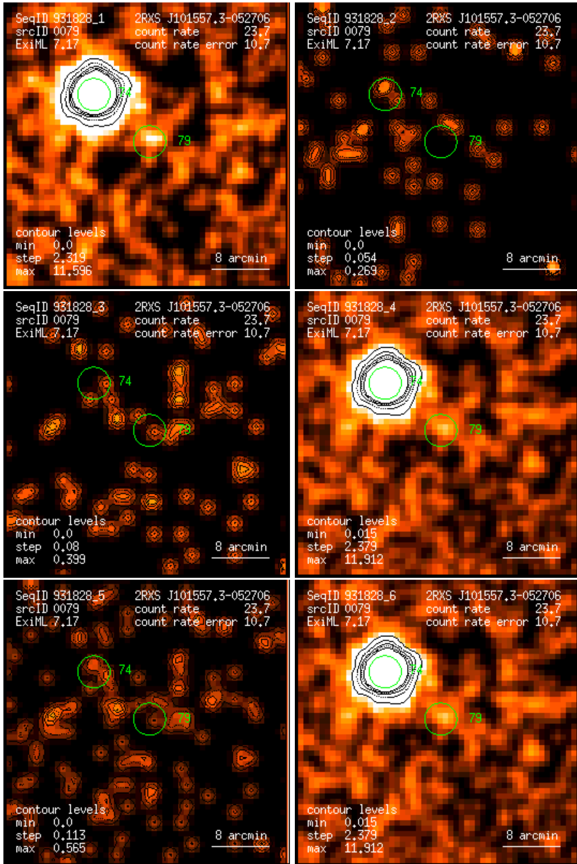
Figure 79: RASS 931828: detection 0079: band rate images, Gaussian filter: (1) PSPC channels 11 – 41, (2) 52 – 90, (3) 91 – 201, (4) 11 – 235, (5) 52 – 201, (6) 11 – 201. Broad band rates in counts/ks. Band rate contour levels in counts/ks/arcmin 2 .
