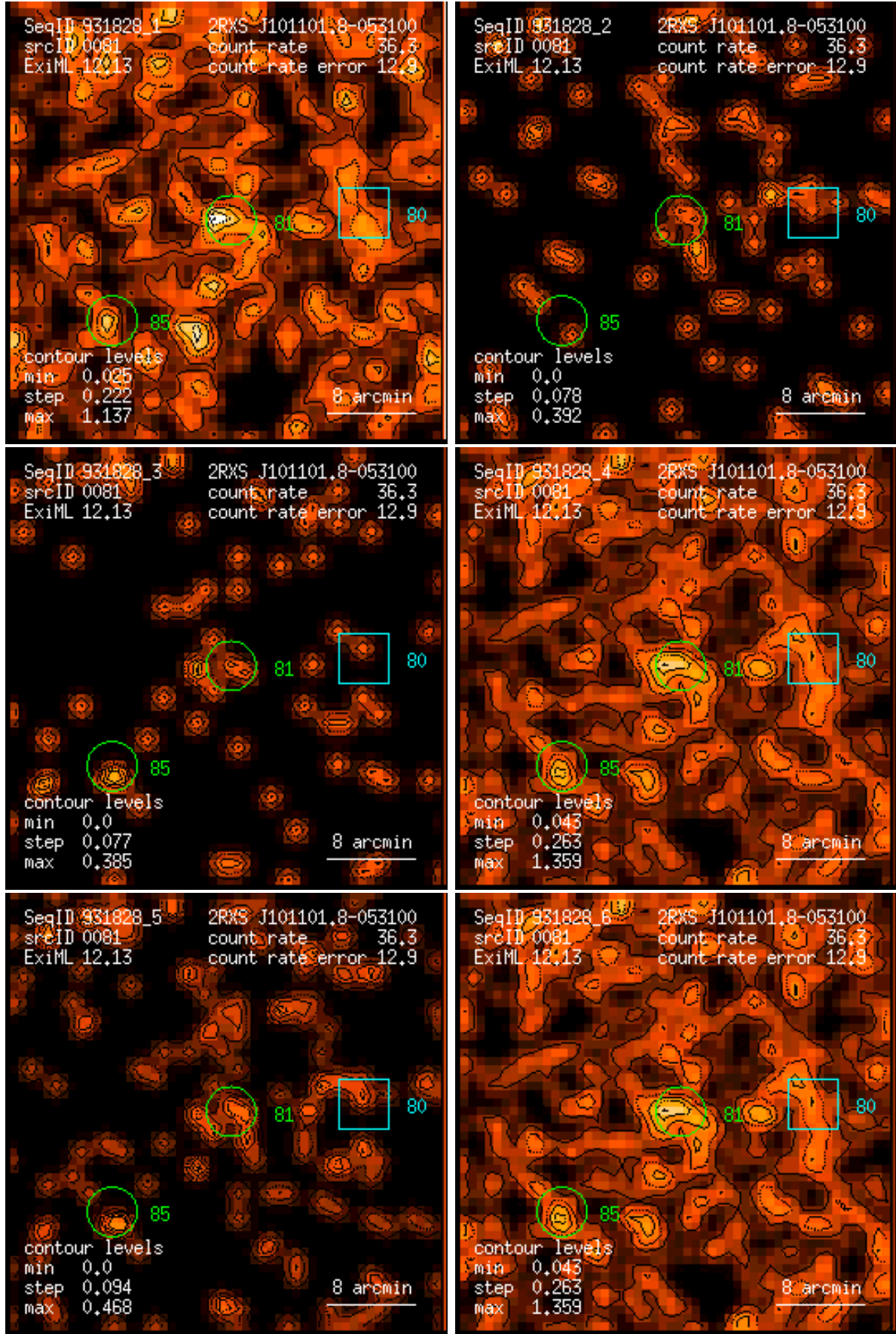
Figure 81: RASS 931828: detection 0081: band rate images, Gaussian filter: (1) PSPC channels 11 – 41, (2) 52 – 90, (3) 91 – 201, (4) 11 – 235, (5) 52 – 201, (6) 11 – 201. Broad band rates in counts/ks. Band rate contour levels in counts/ks/arcmin 2 .
