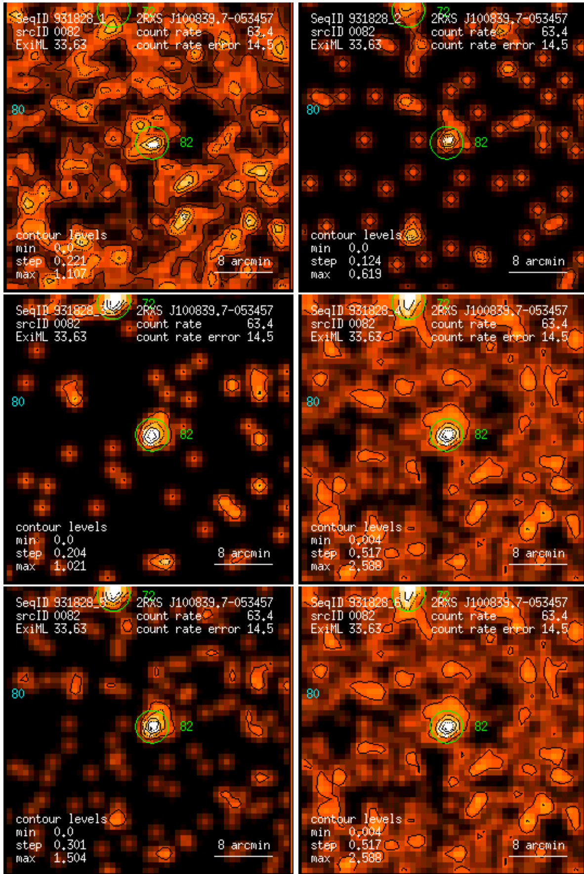
Figure 82: RASS 931828: detection 0082: band rate images, Gaussian filter: (1) PSPC channels 11 – 41, (2) 52 – 90, (3) 91 – 201, (4) 11 – 235, (5) 52 – 201, (6) 11 – 201. Broad band rates in counts/ks. Band rate contour levels in counts/ks/arcmin 2 .
