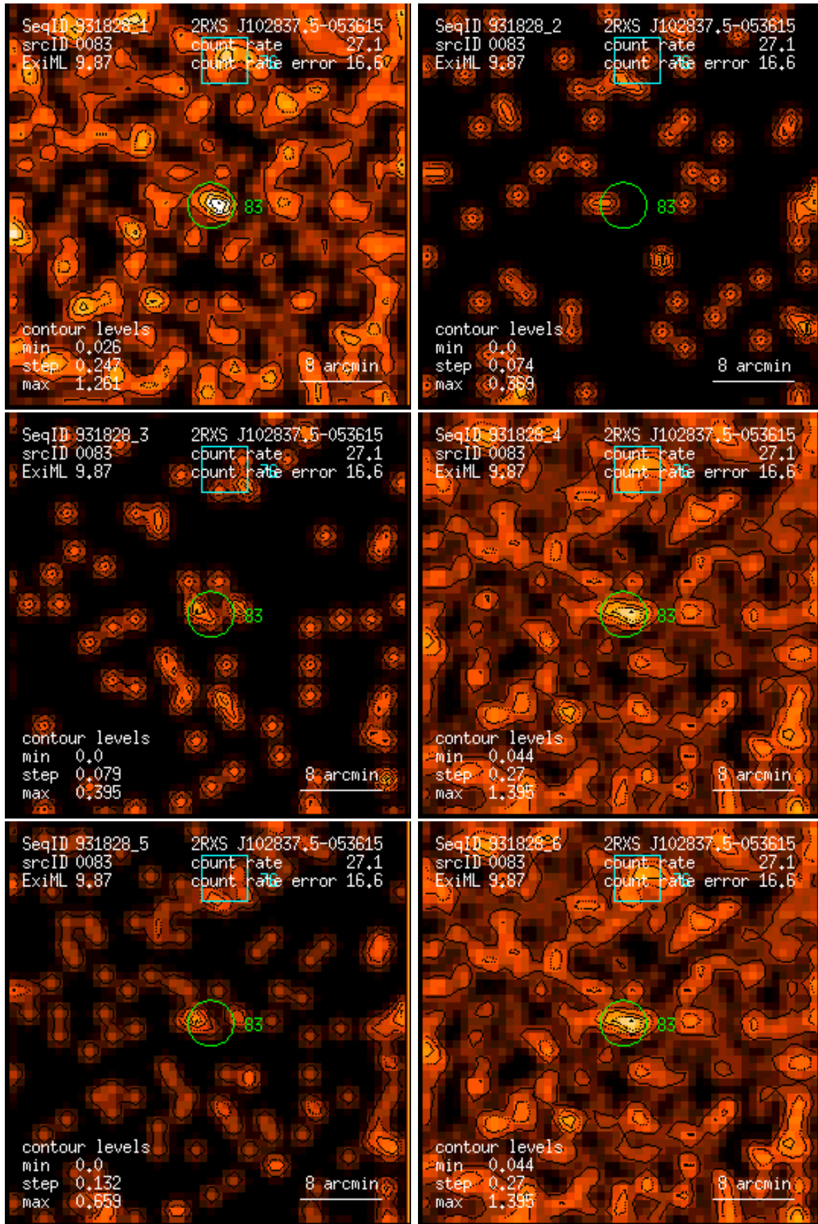
Figure 83: RASS 931828: detection 0083: band rate images, Gaussian filter: (1) PSPC channels 11 – 41, (2) 52 – 90, (3) 91 – 201, (4) 11 – 235, (5) 52 – 201, (6) 11 – 201. Broad band rates in counts/ks. Band rate contour levels in counts/ks/arcmin 2 .
