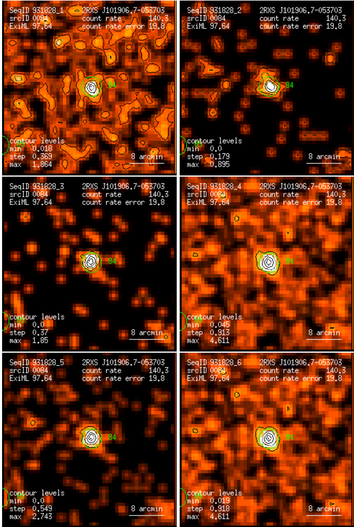
Figure 84: RASS 931828: detection 0084: band rate images, Gaussian filter: (1) PSPC channels 11 – 41, (2) 52 – 90, (3) 91 – 201, (4) 11 – 235, (5) 52 – 201, (6) 11 – 201. Broad band rates in counts/ks. Band rate contour levels in counts/ks/arcmin 2 .
