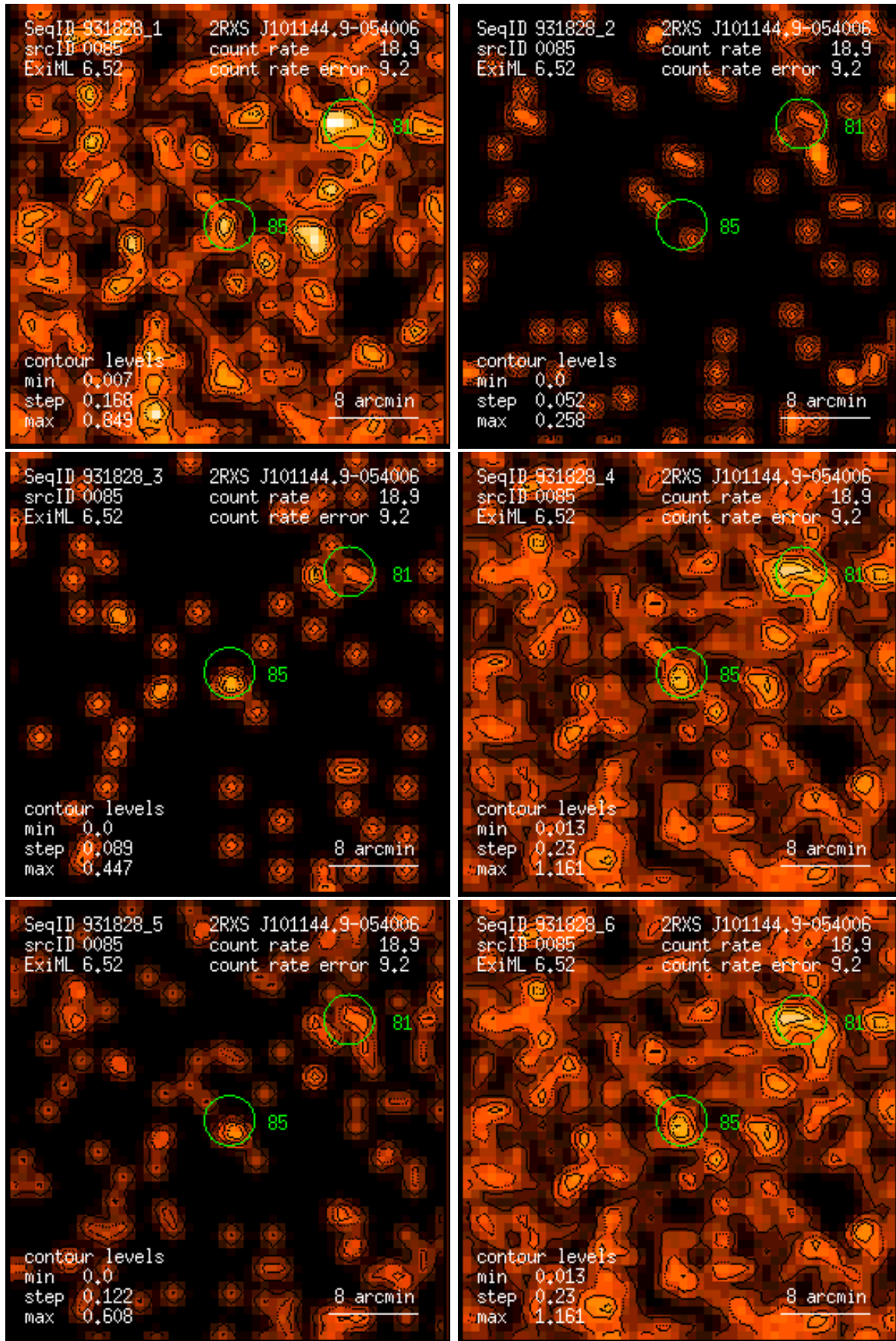
Figure 85: RASS 931828: detection 0085: band rate images, Gaussian filter: (1) PSPC channels 11 – 41, (2) 52 – 90, (3) 91 – 201, (4) 11 – 235, (5) 52 – 201, (6) 11 – 201. Broad band rates in counts/ks. Band rate contour levels in counts/ks/arcmin 2 .
