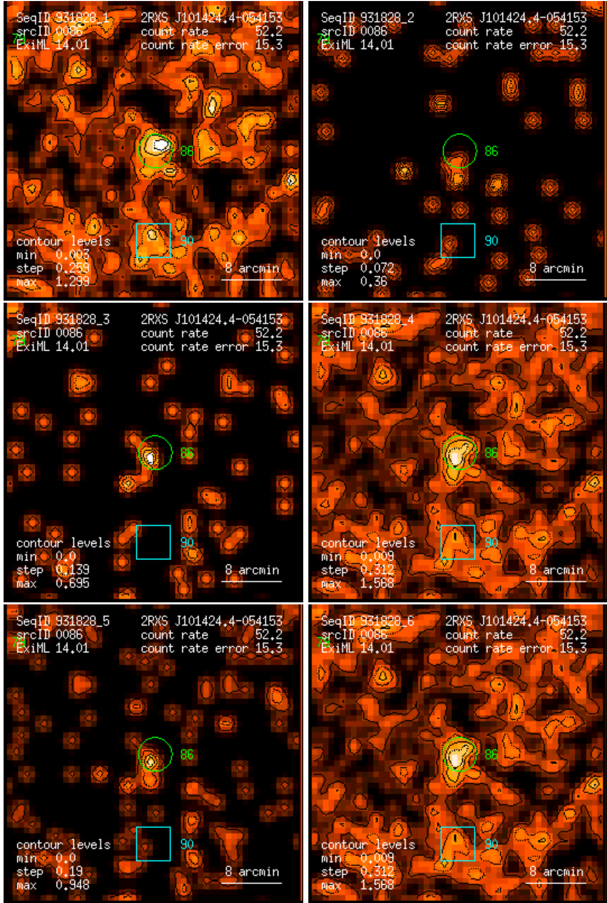
Figure 86: RASS 931828: detection 0086: band rate images, Gaussian filter: (1) PSPC channels 11 – 41, (2) 52 – 90, (3) 91 – 201, (4) 11 – 235, (5) 52 – 201, (6) 11 – 201. Broad band rates in counts/ks. Band rate contour levels in counts/ks/arcmin 2 .
