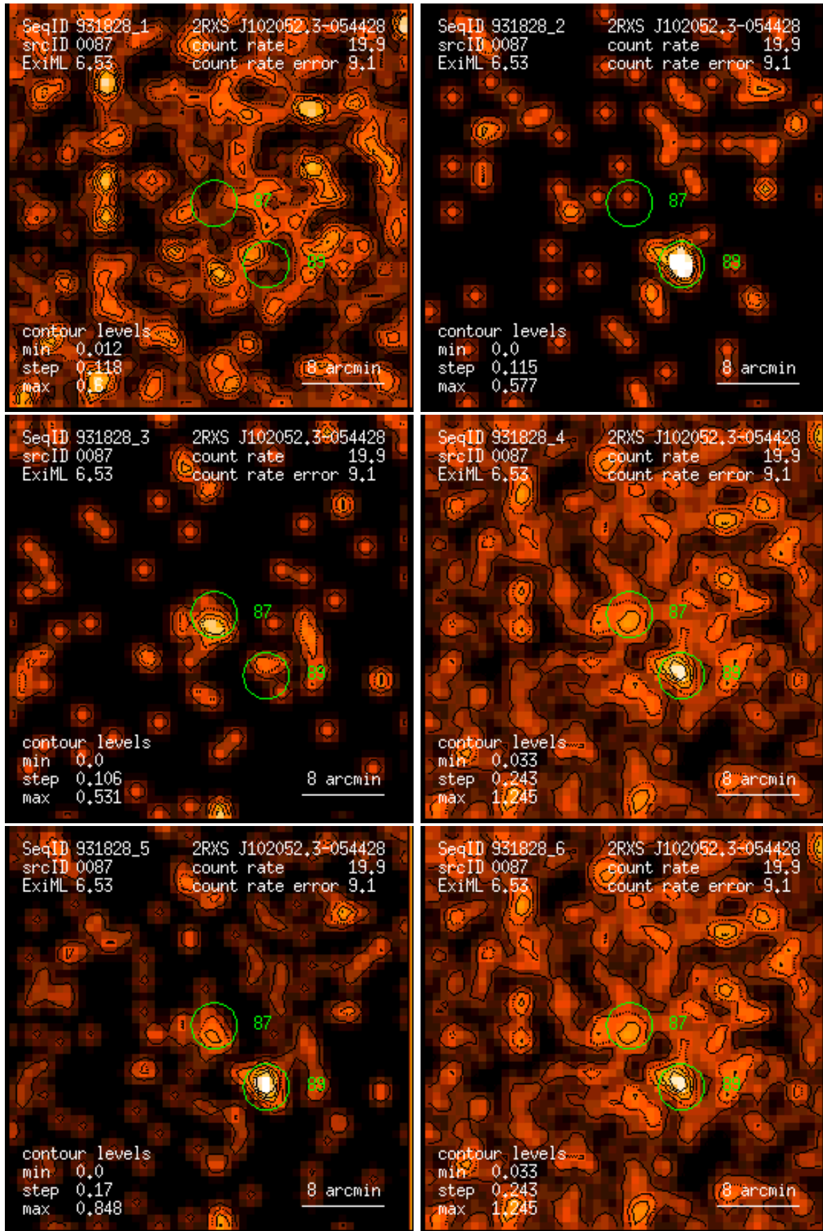
Figure 87: RASS 931828: detection 0087: band rate images, Gaussian filter: (1) PSPC channels 11 – 41, (2) 52 – 90, (3) 91 – 201, (4) 11 – 235, (5) 52 – 201, (6) 11 – 201. Broad band rates in counts/ks. Band rate contour levels in counts/ks/arcmin 2 .
