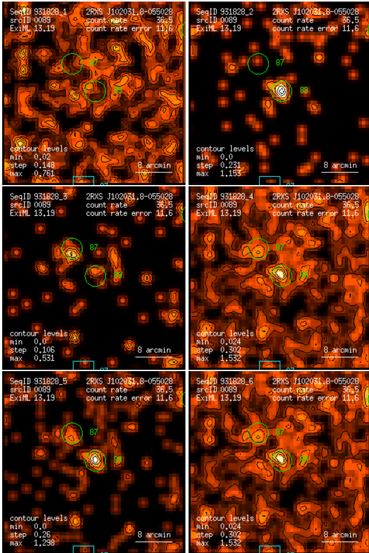
Figure 89: RASS 931828: detection 0089: band rate images, Gaussian filter: (1) PSPC channels 11 – 41, (2) 52 – 90, (3) 91 – 201, (4) 11 – 235, (5) 52 – 201, (6) 11 – 201. Broad band rates in counts/ks. Band rate contour levels in counts/ks/arcmin 2 .
