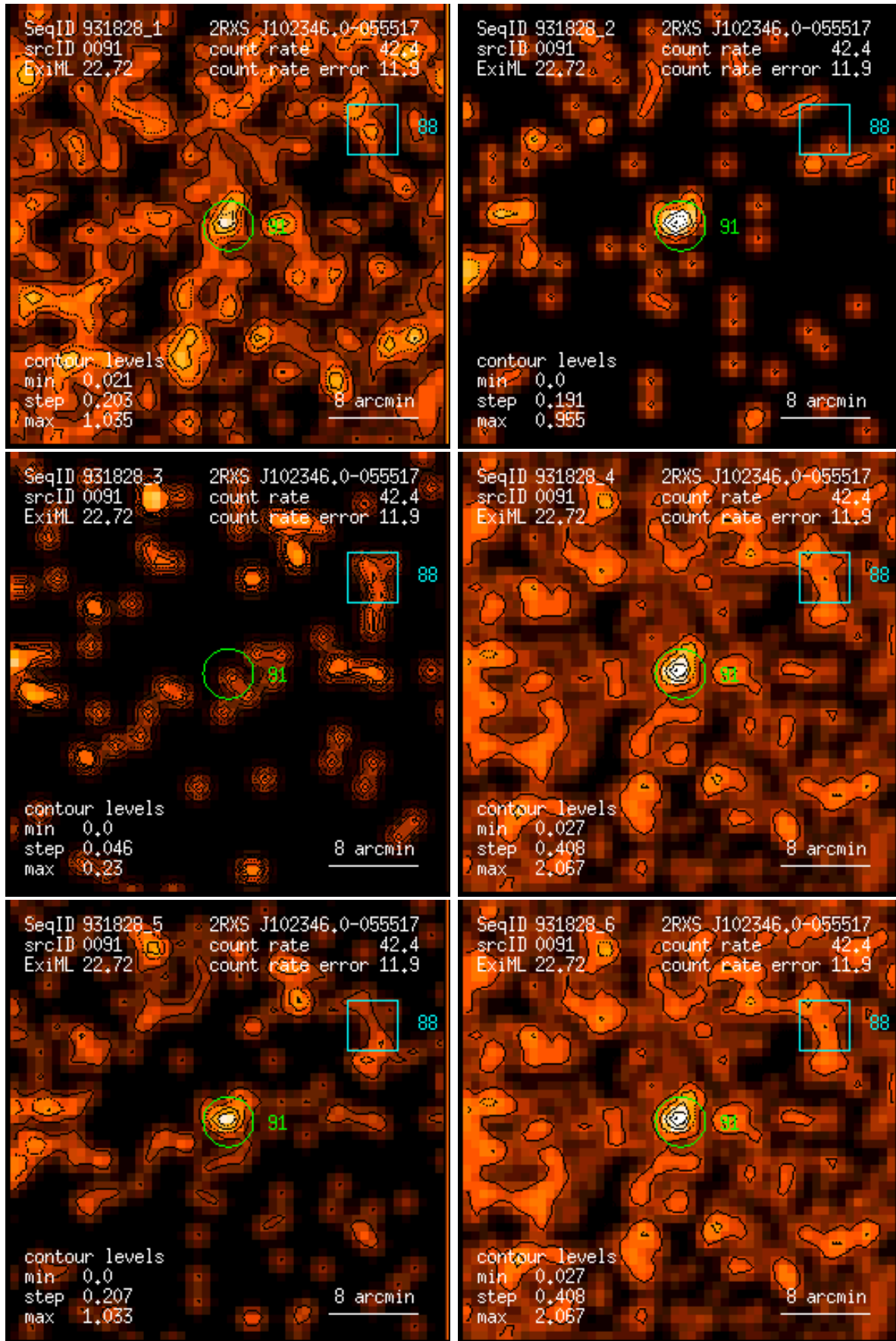
Figure 91: RASS 931828: detection 0091: band rate images, Gaussian filter: (1) PSPC channels 11 – 41, (2) 52 – 90, (3) 91 – 201, (4) 11 – 235, (5) 52 – 201, (6) 11 – 201. Broad band rates in counts/ks. Band rate contour levels in counts/ks/arcmin 2 .
