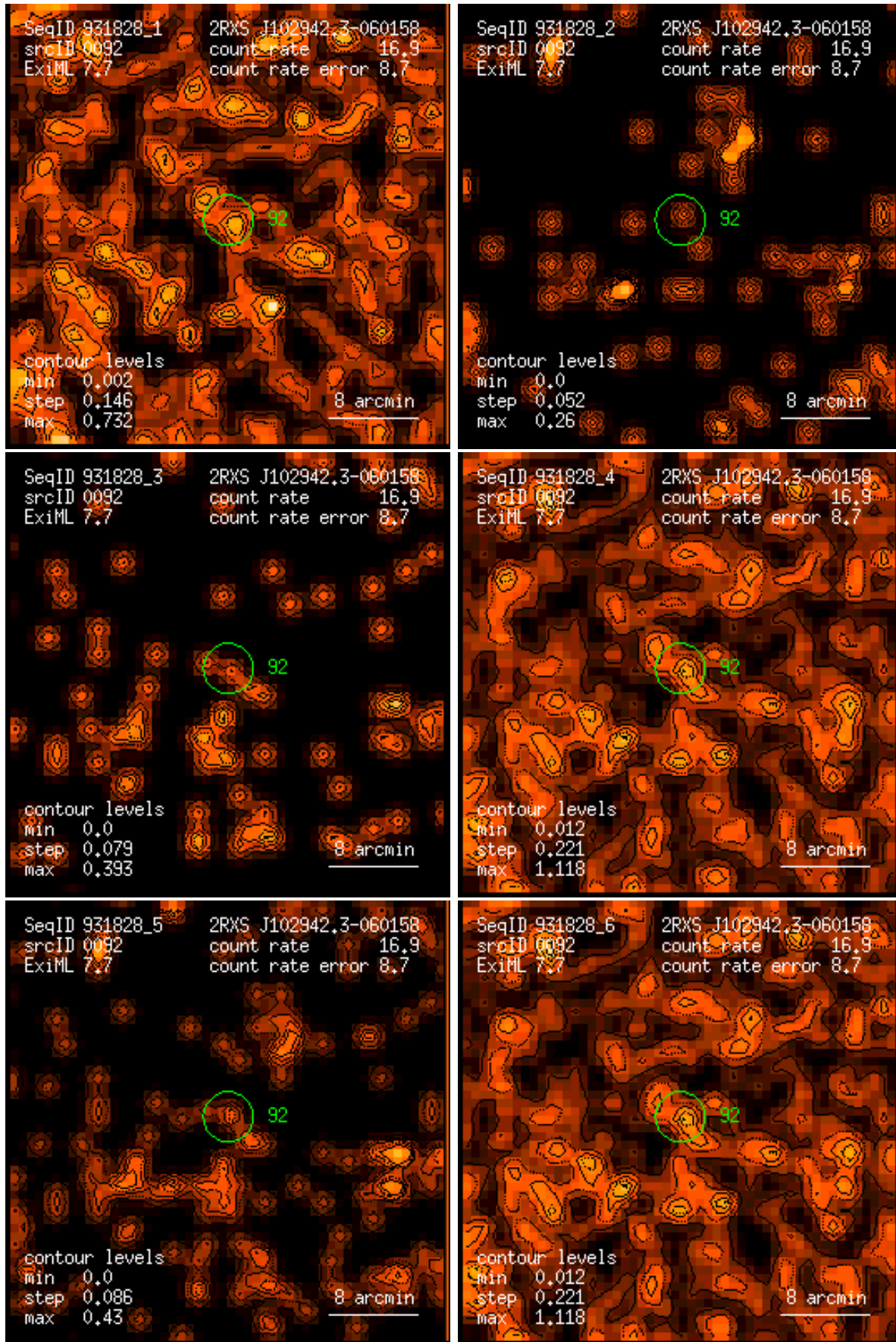
Figure 92: RASS 931828: detection 0092: band rate images, Gaussian filter: (1) PSPC channels 11 – 41, (2) 52 – 90, (3) 91 – 201, (4) 11 – 235, (5) 52 – 201, (6) 11 – 201. Broad band rates in counts/ks. Band rate contour levels in counts/ks/arcmin 2 .
