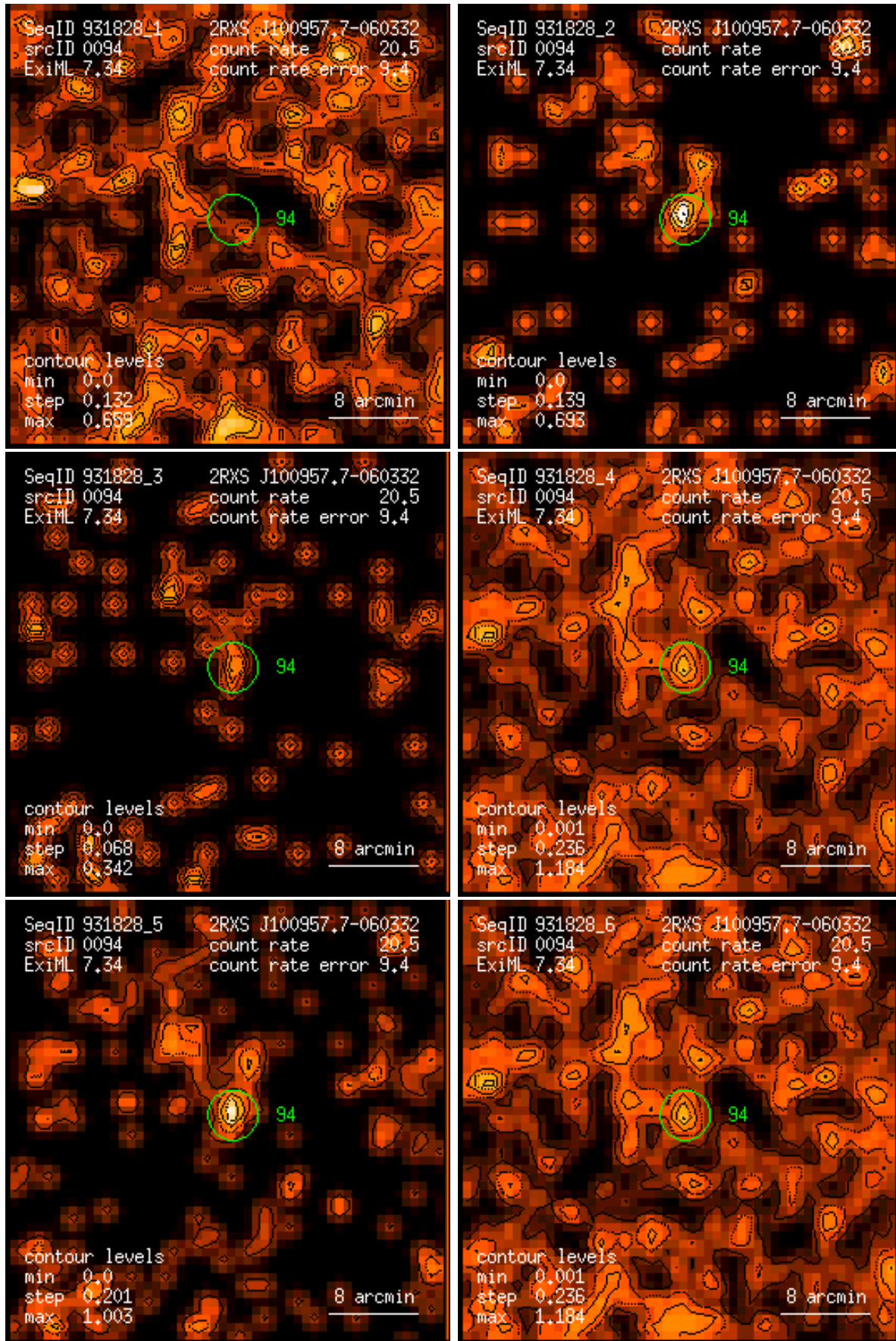
Figure 94: RASS 931828: detection 0094: band rate images, Gaussian filter: (1) PSPC channels 11 – 41, (2) 52 – 90, (3) 91 – 201, (4) 11 – 235, (5) 52 – 201, (6) 11 – 201. Broad band rates in counts/ks. Band rate contour levels in counts/ks/arcmin 2 .
