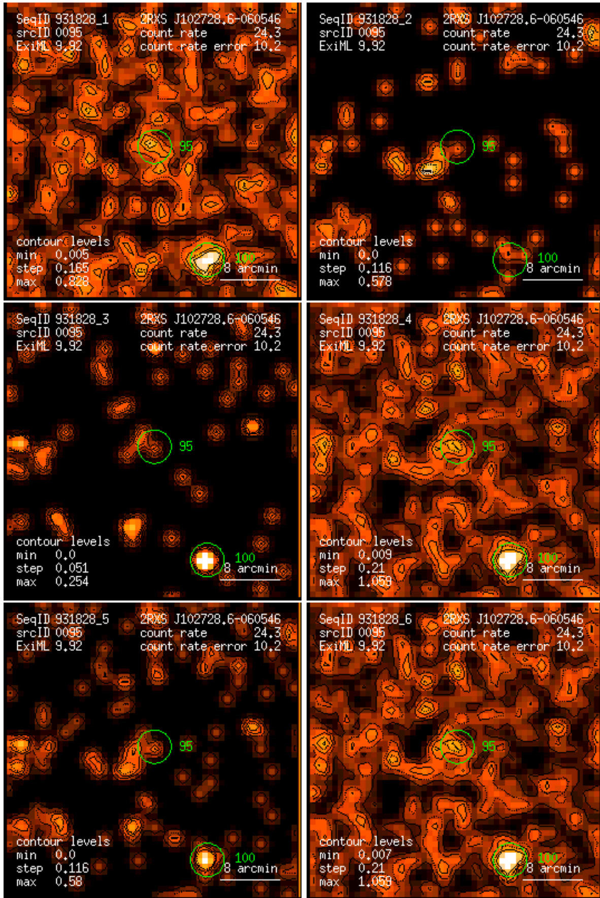
Figure 95: RASS 931828: detection 0095: band rate images, Gaussian filter: (1) PSPC channels 11 – 41, (2) 52 – 90, (3) 91 – 201, (4) 11 – 235, (5) 52 – 201, (6) 11 – 201. Broad band rates in counts/ks. Band rate contour levels in counts/ks/arcmin 2 .
