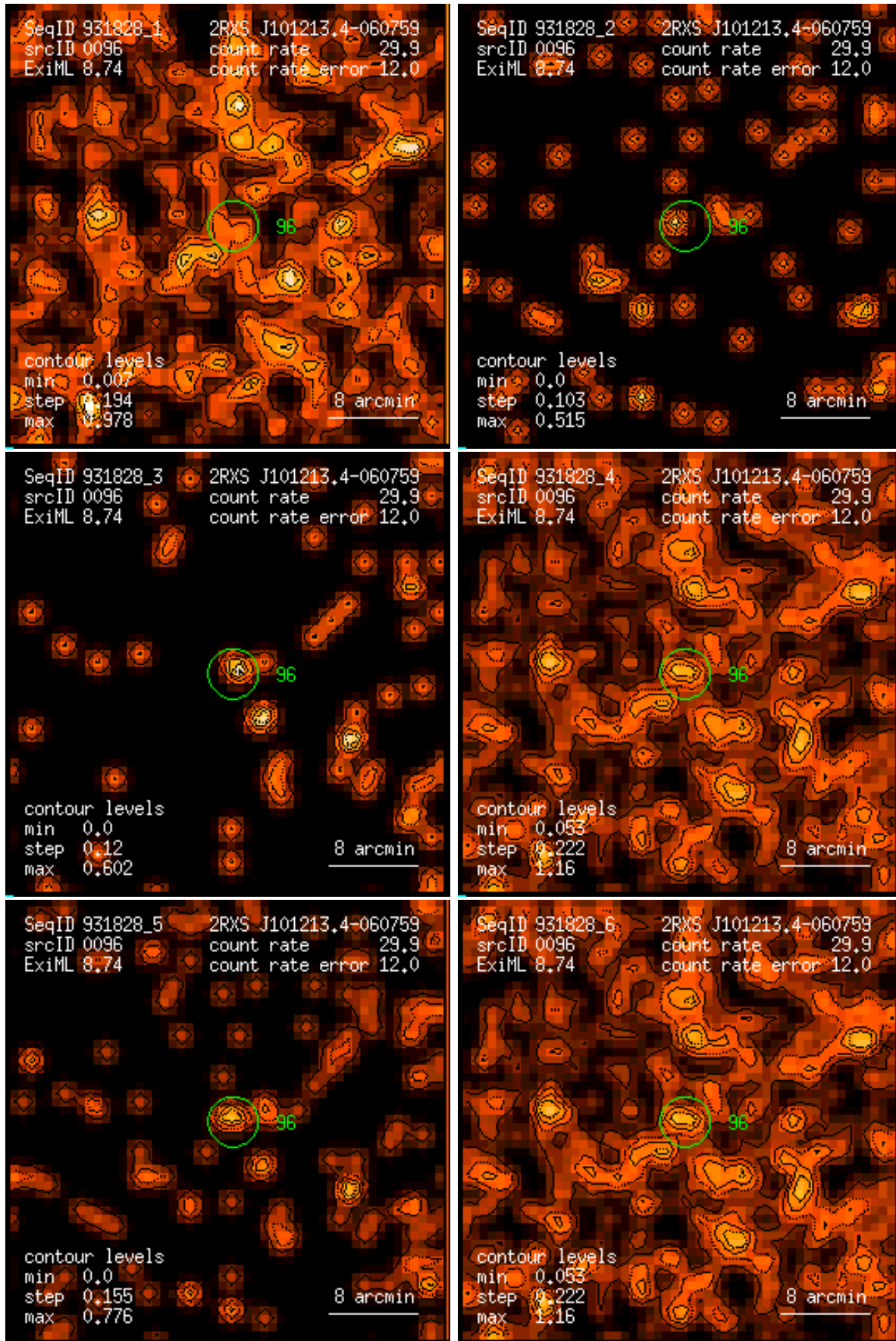
Figure 96: RASS 931828: detection 0096: band rate images, Gaussian filter: (1) PSPC channels 11 – 41, (2) 52 – 90, (3) 91 – 201, (4) 11 – 235, (5) 52 – 201, (6) 11 – 201. Broad band rates in counts/ks. Band rate contour levels in counts/ks/arcmin 2 .
