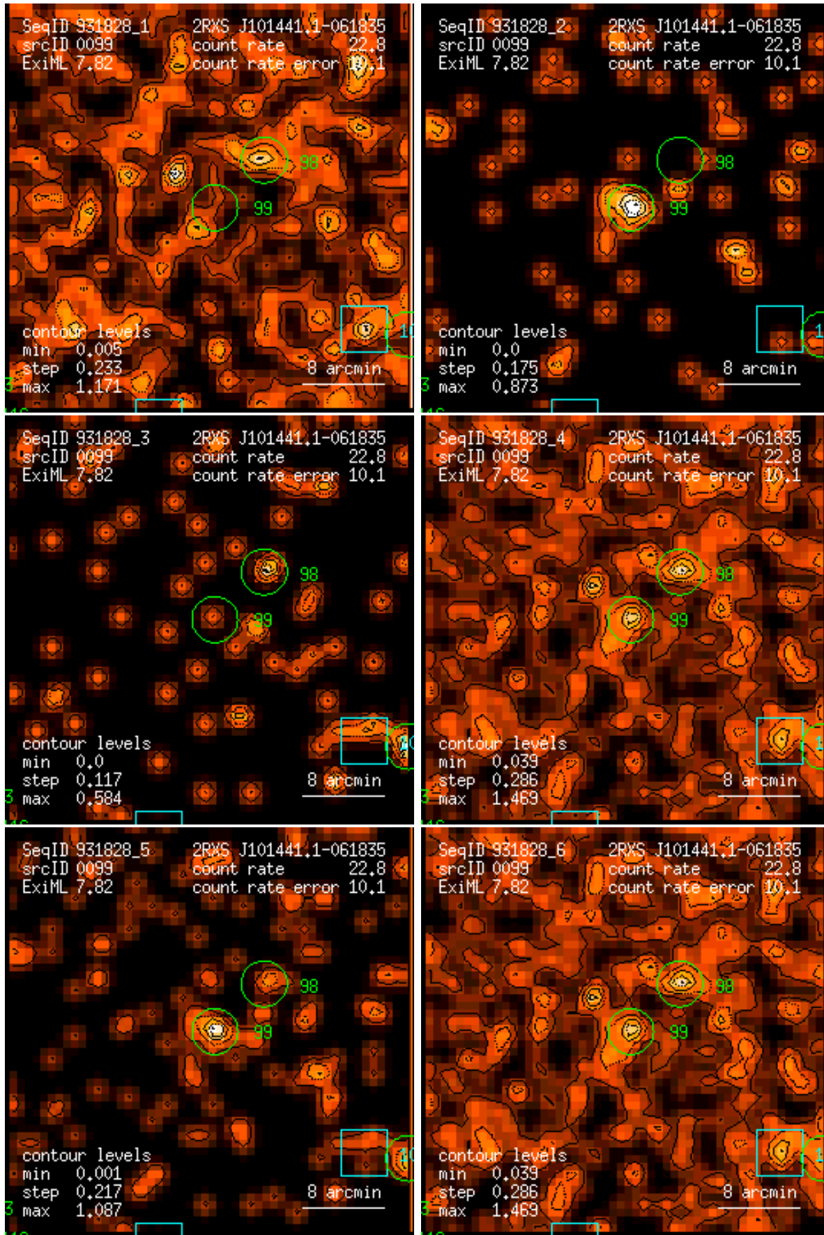
Figure 99: RASS 931828: detection 0099: band rate images, Gaussian filter: (1) PSPC channels 11 – 41, (2) 52 – 90, (3) 91 – 201, (4) 11 – 235, (5) 52 – 201, (6) 11 – 201. Broad band rates in counts/ks. Band rate contour levels in counts/ks/arcmin 2 .
